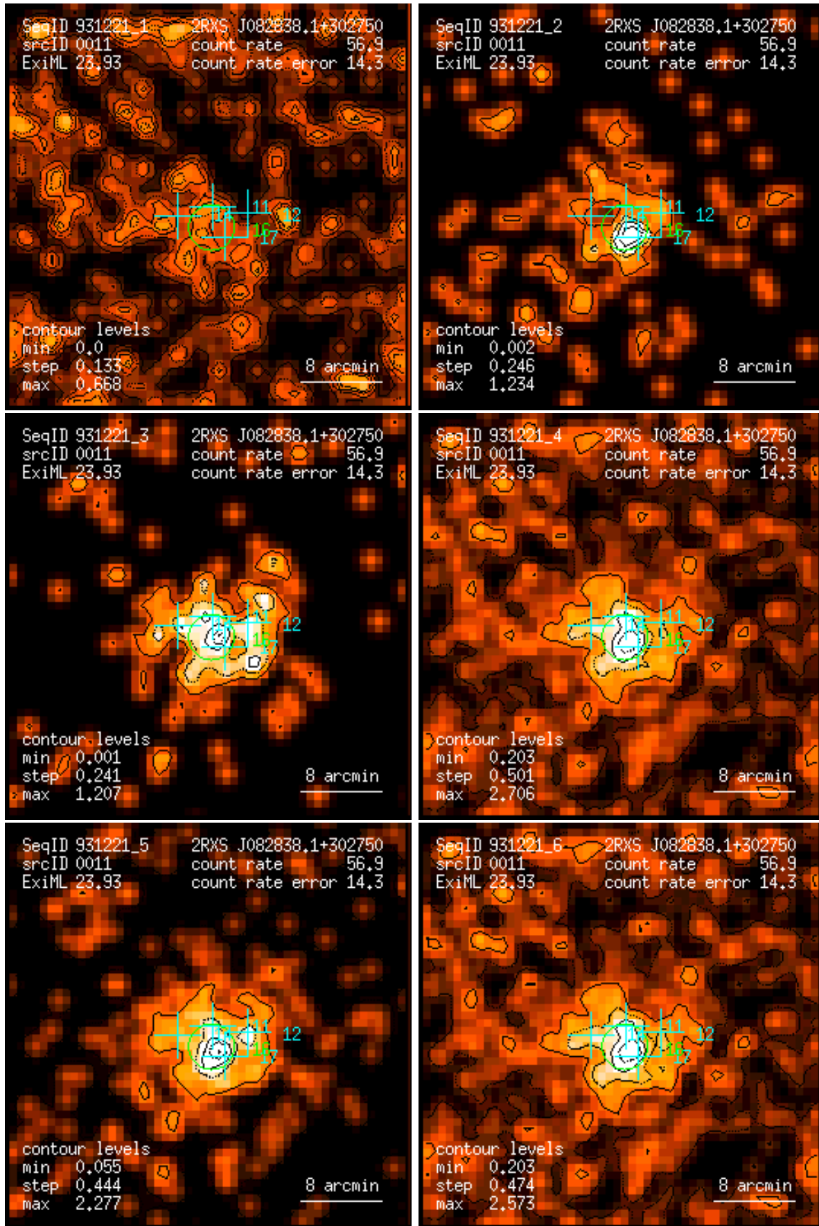
Figure 11: RASS 931221: detection 0011: band rate images, Gaussian filter: (1) PSPC channels 11 – 41, (2) 52 – 90, (3) 91 – 201, (4) 11 – 235, (5) 52 – 201, (6) 11 – 201. Broad band rates in counts/ks. Band rate contour levels in counts/ks/arcmin 2 .
