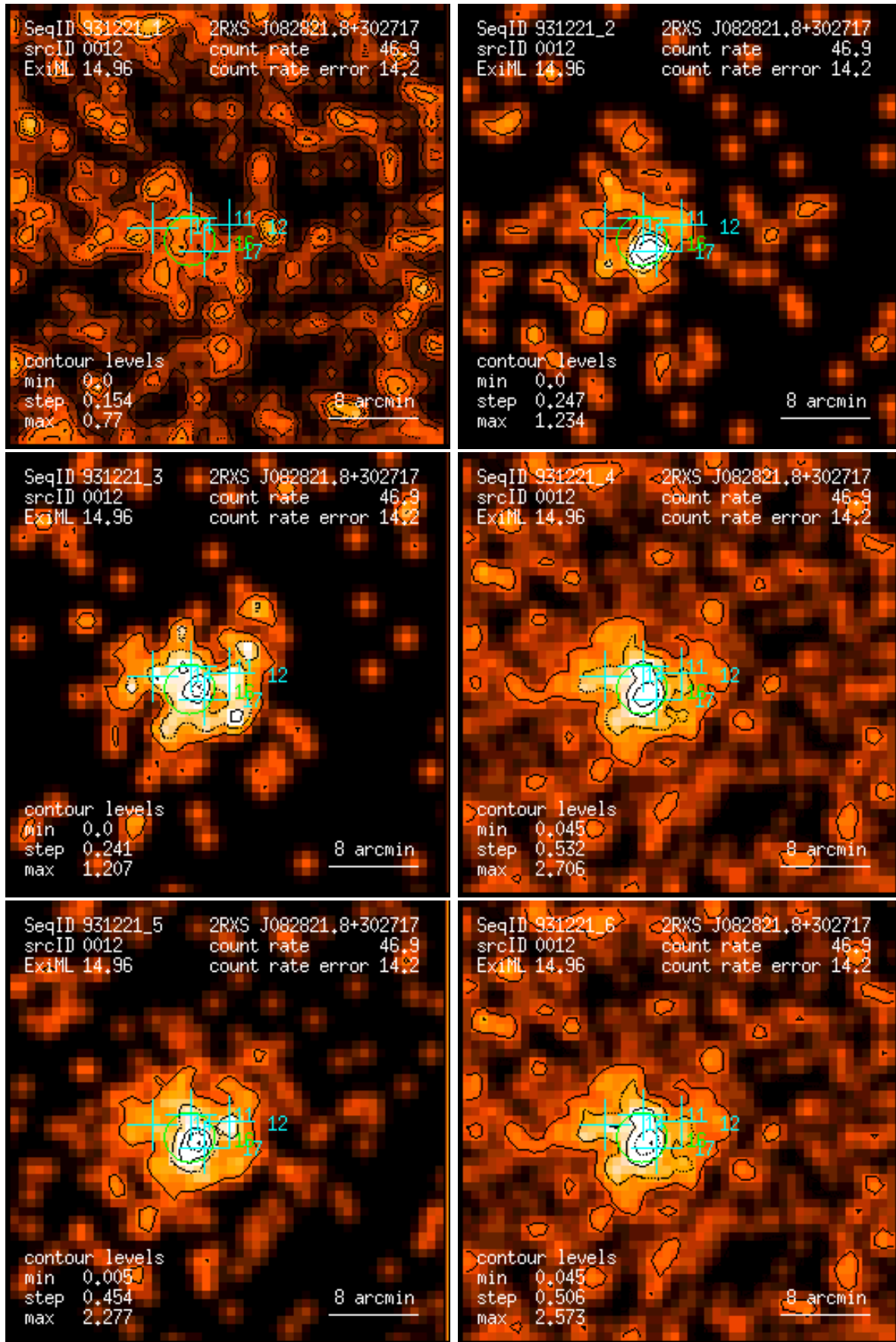
Figure 12: RASS 931221: detection 0012: band rate images, Gaussian filter: (1) PSPC channels 11 – 41, (2) 52 – 90, (3) 91 – 201, (4) 11 – 235, (5) 52 – 201, (6) 11 – 201. Broad band rates in counts/ks. Band rate contour levels in counts/ks/arcmin 2 .
