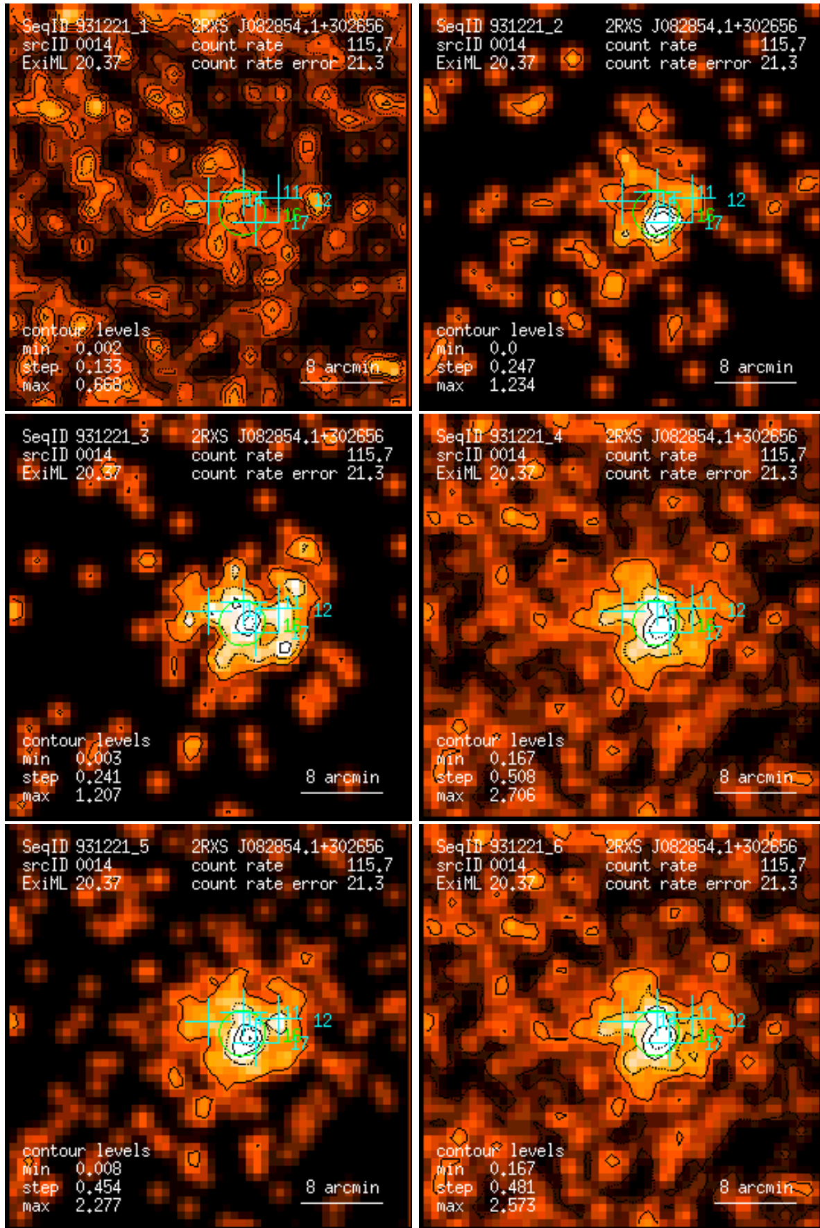
Figure 14: RASS 931221: detection 0014: band rate images, Gaussian filter: (1) PSPC channels 11 – 41, (2) 52 – 90, (3) 91 – 201, (4) 11 – 235, (5) 52 – 201, (6) 11 – 201. Broad band rates in counts/ks. Band rate contour levels in counts/ks/arcmin 2 .
