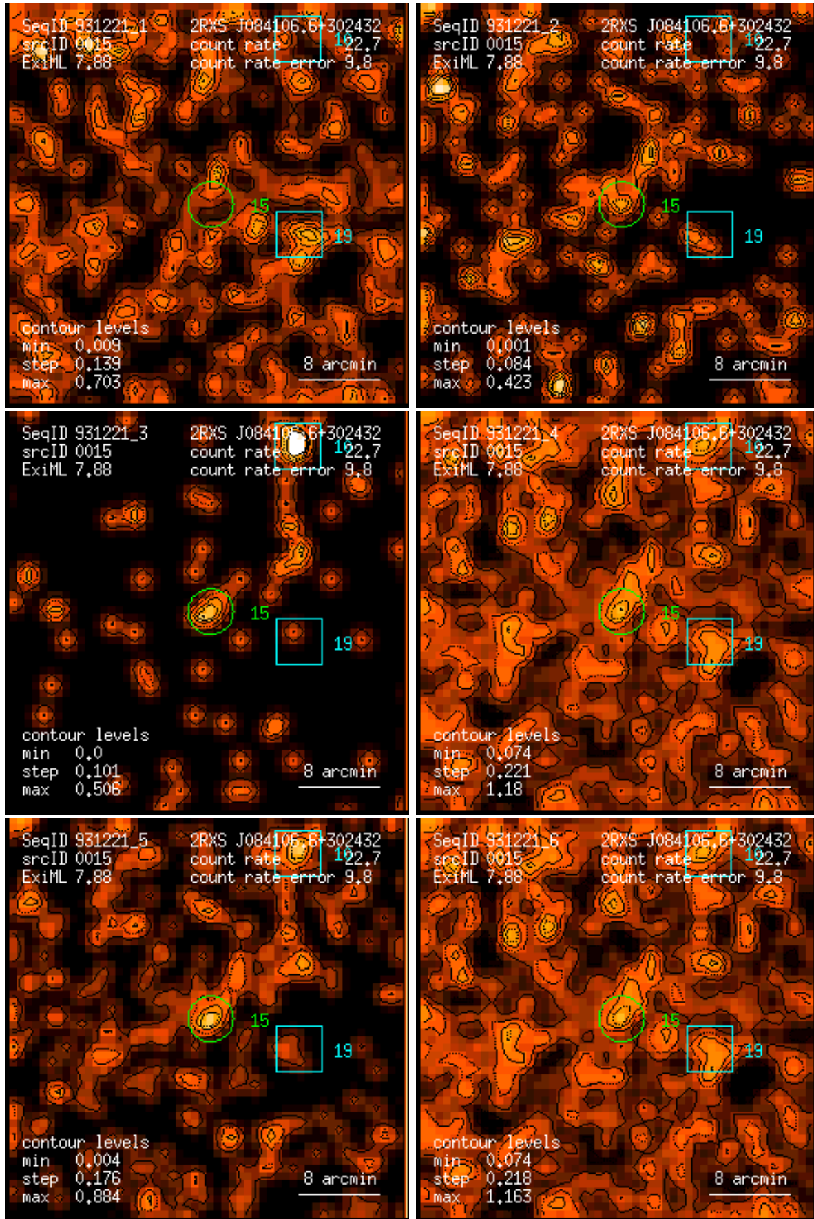
Figure 15: RASS 931221: detection 0015: band rate images, Gaussian filter: (1) PSPC channels 11 – 41, (2) 52 – 90, (3) 91 – 201, (4) 11 – 235, (5) 52 – 201, (6) 11 – 201. Broad band rates in counts/ks. Band rate contour levels in counts/ks/arcmin 2 .
