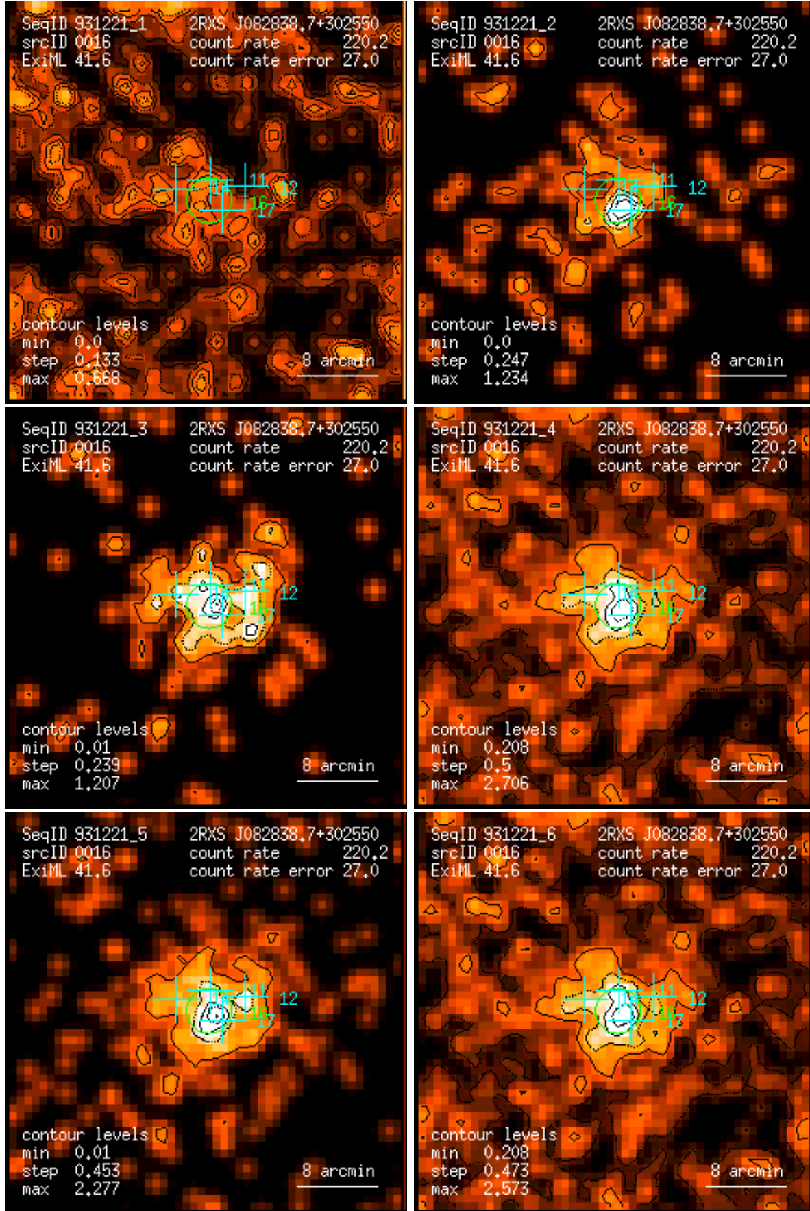
Figure 16: RASS 931221: detection 0016: band rate images, Gaussian filter: (1) PSPC channels 11 – 41, (2) 52 – 90, (3) 91 – 201, (4) 11 – 235, (5) 52 – 201, (6) 11 – 201. Broad band rates in counts/ks. Band rate contour levels in counts/ks/arcmin 2 .
