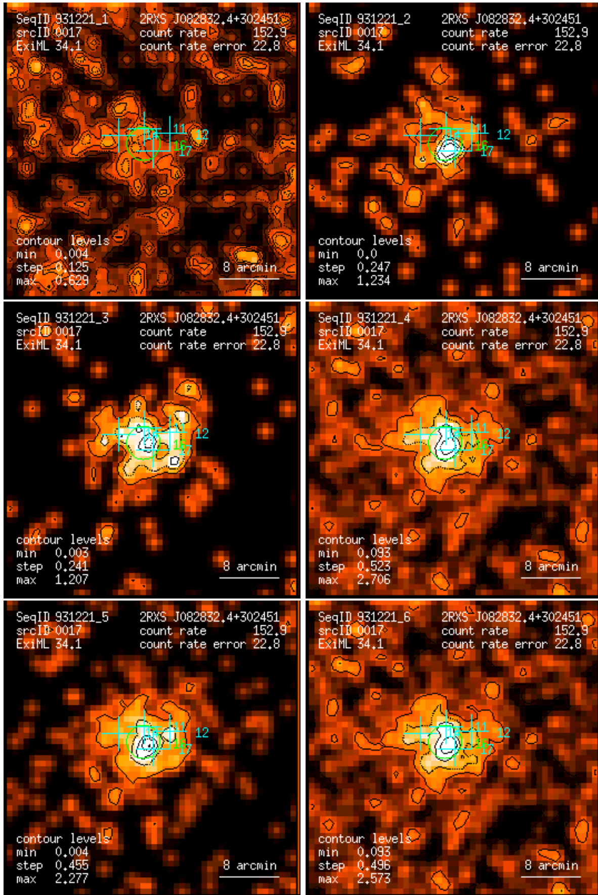
Figure 17: RASS 931221: detection 0017: band rate images, Gaussian filter: (1) PSPC channels 11 – 41, (2) 52 – 90, (3) 91 – 201, (4) 11 – 235, (5) 52 – 201, (6) 11 – 201. Broad band rates in counts/ks. Band rate contour levels in counts/ks/arcmin 2 .
