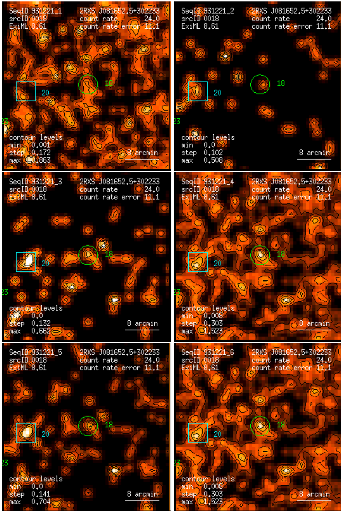
Figure 18: RASS 931221: detection 0018: band rate images, Gaussian filter: (1) PSPC channels 11 – 41, (2) 52 – 90, (3) 91 – 201, (4) 11 – 235, (5) 52 – 201, (6) 11 – 201. Broad band rates in counts/ks. Band rate contour levels in counts/ks/arcmin 2 .
