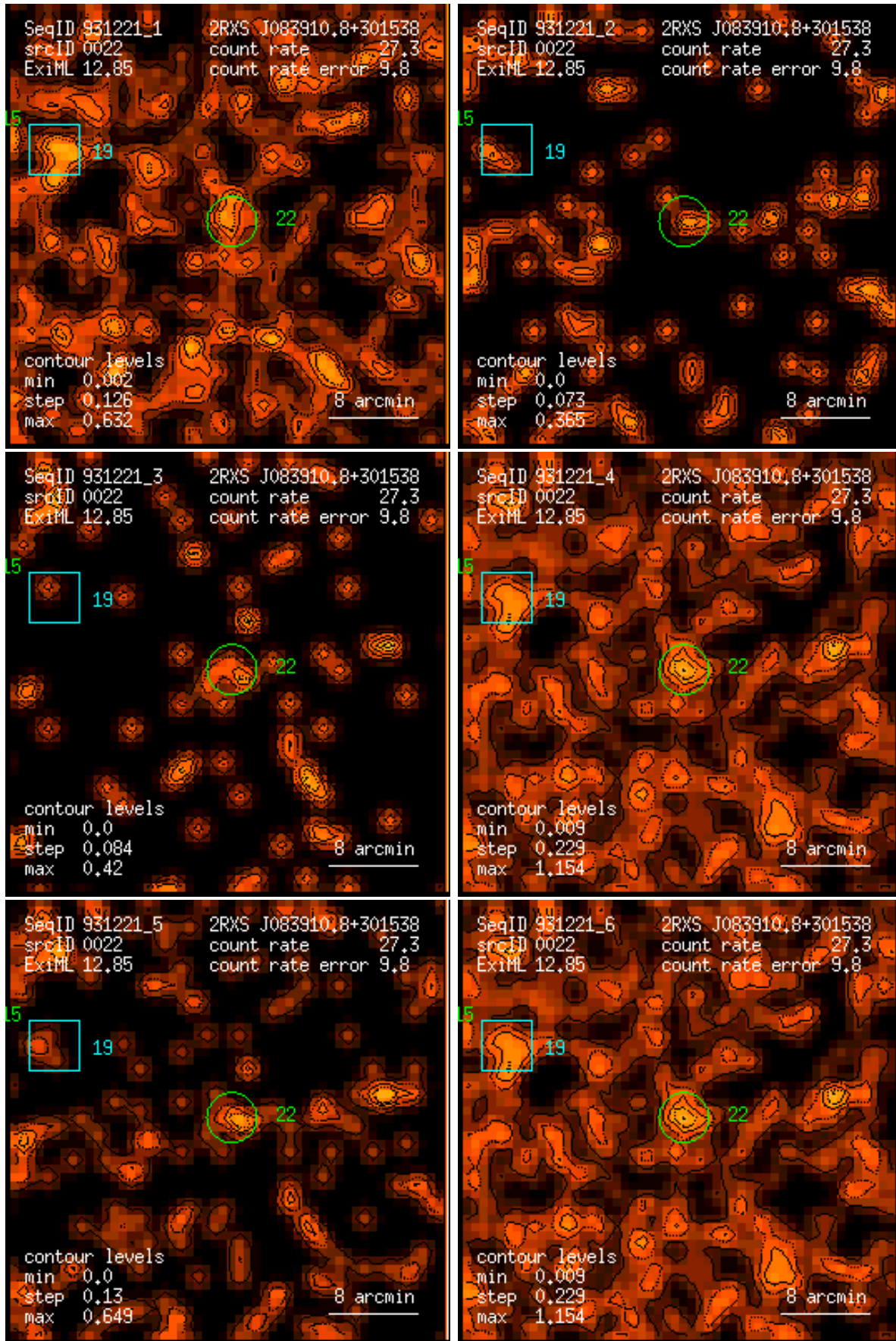
Figure 22: RASS 931221: detection 0022: band rate images, Gaussian filter: (1) PSPC channels 11 – 41, (2) 52 – 90, (3) 91 – 201, (4) 11 – 235, (5) 52 – 201, (6) 11 – 201. Broad band rates in counts/ks. Band rate contour levels in counts/ks/arcmin 2 .
