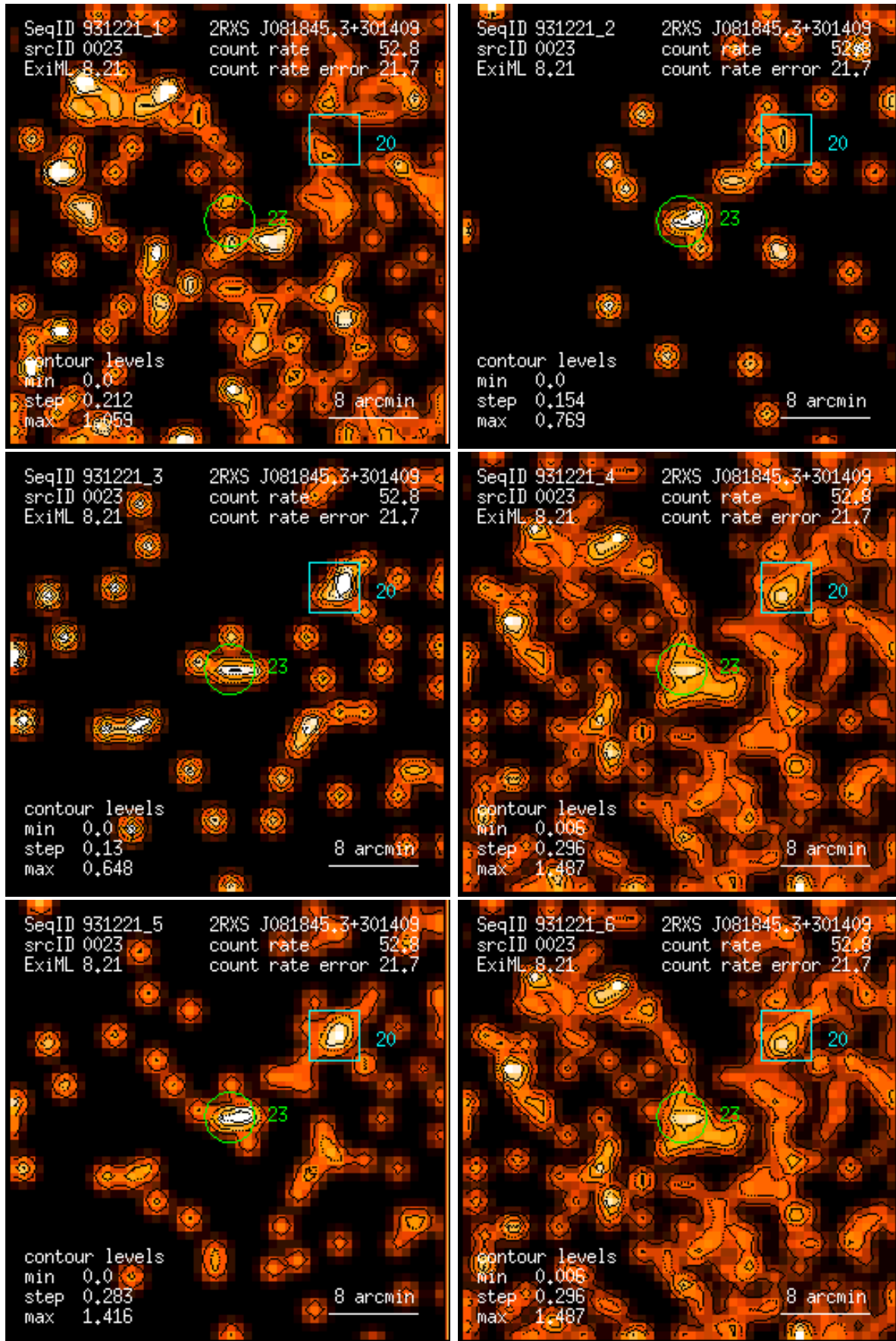
Figure 23: RASS 931221: detection 0023: band rate images, Gaussian filter: (1) PSPC channels 11 – 41, (2) 52 – 90, (3) 91 – 201, (4) 11 – 235, (5) 52 – 201, (6) 11 – 201. Broad band rates in counts/ks. Band rate contour levels in counts/ks/arcmin 2 .
