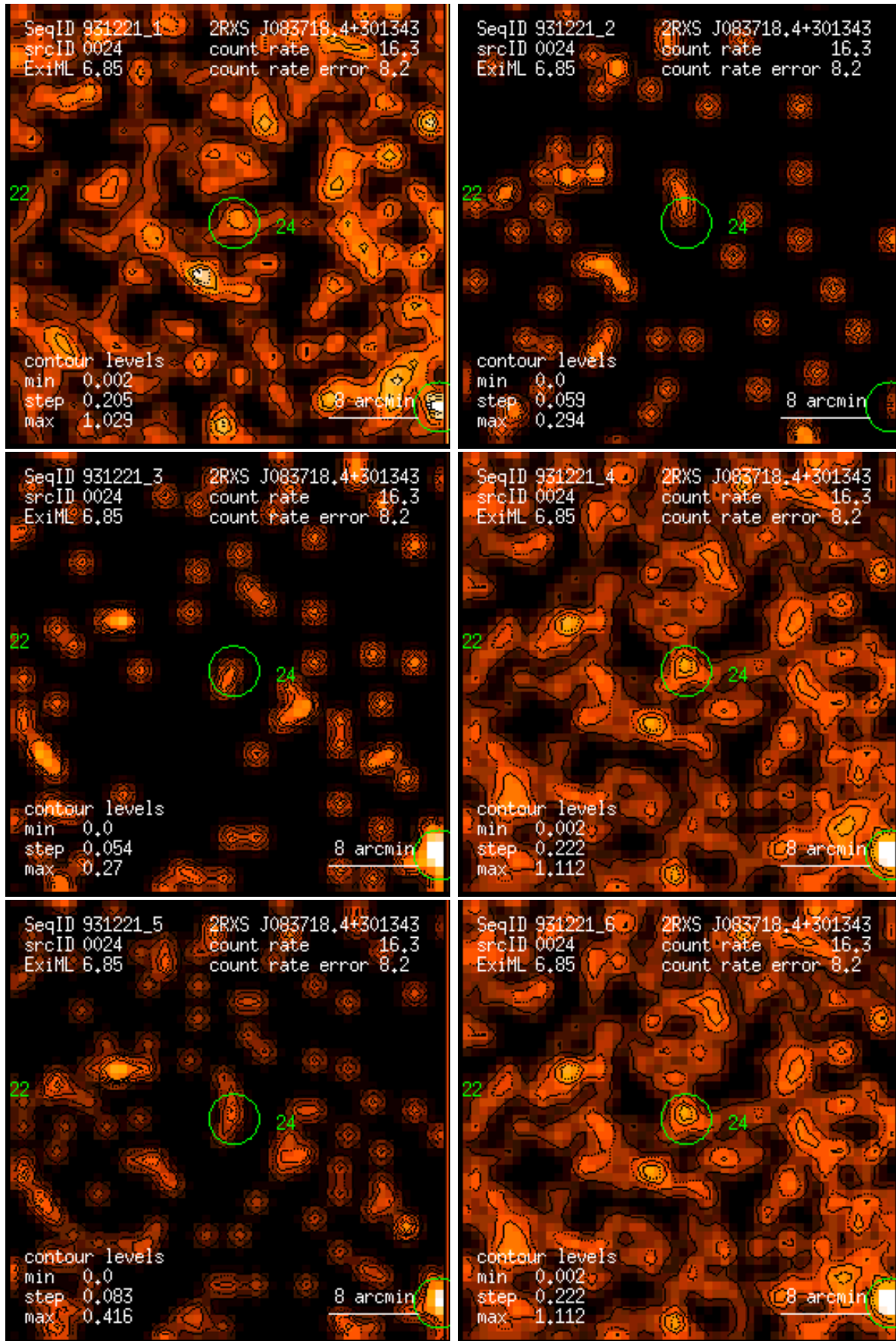
Figure 24: RASS 931221: detection 0024: band rate images, Gaussian filter: (1) PSPC channels 11 – 41, (2) 52 – 90, (3) 91 – 201, (4) 11 – 235, (5) 52 – 201, (6) 11 – 201. Broad band rates in counts/ks. Band rate contour levels in counts/ks/arcmin 2 .
