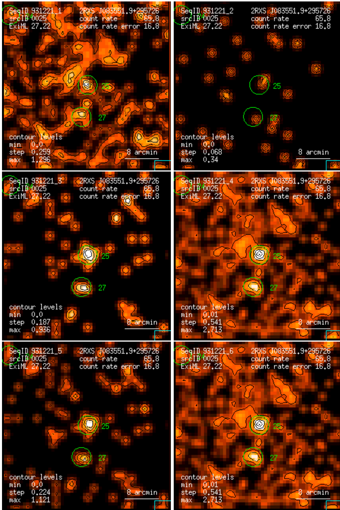
Figure 25: RASS 931221: detection 0025: band rate images, Gaussian filter: (1) PSPC channels 11 – 41, (2) 52 – 90, (3) 91 – 201, (4) 11 – 235, (5) 52 – 201, (6) 11 – 201. Broad band rates in counts/ks. Band rate contour levels in counts/ks/arcmin 2 .
