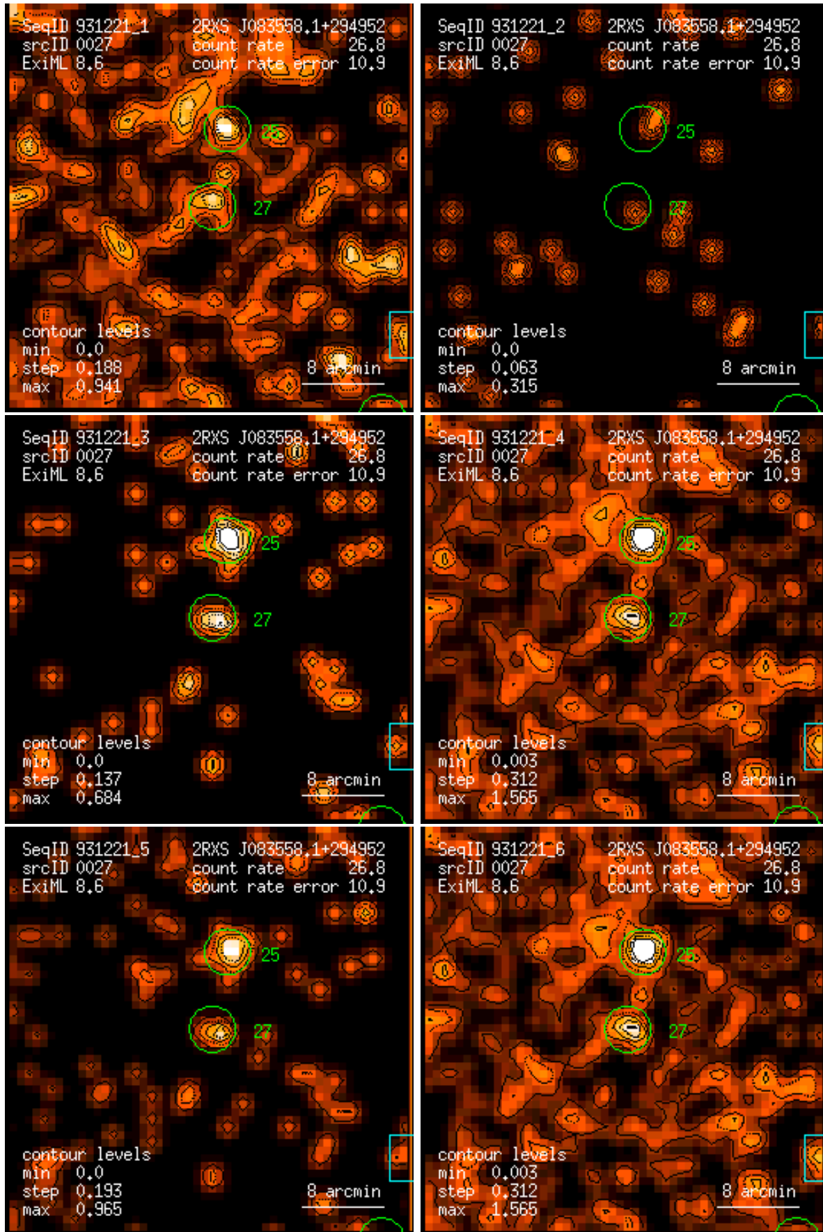
Figure 27: RASS 931221: detection 0027: band rate images, Gaussian filter: (1) PSPC channels 11 – 41, (2) 52 – 90, (3) 91 – 201, (4) 11 – 235, (5) 52 – 201, (6) 11 – 201. Broad band rates in counts/ks. Band rate contour levels in counts/ks/arcmin 2 .
