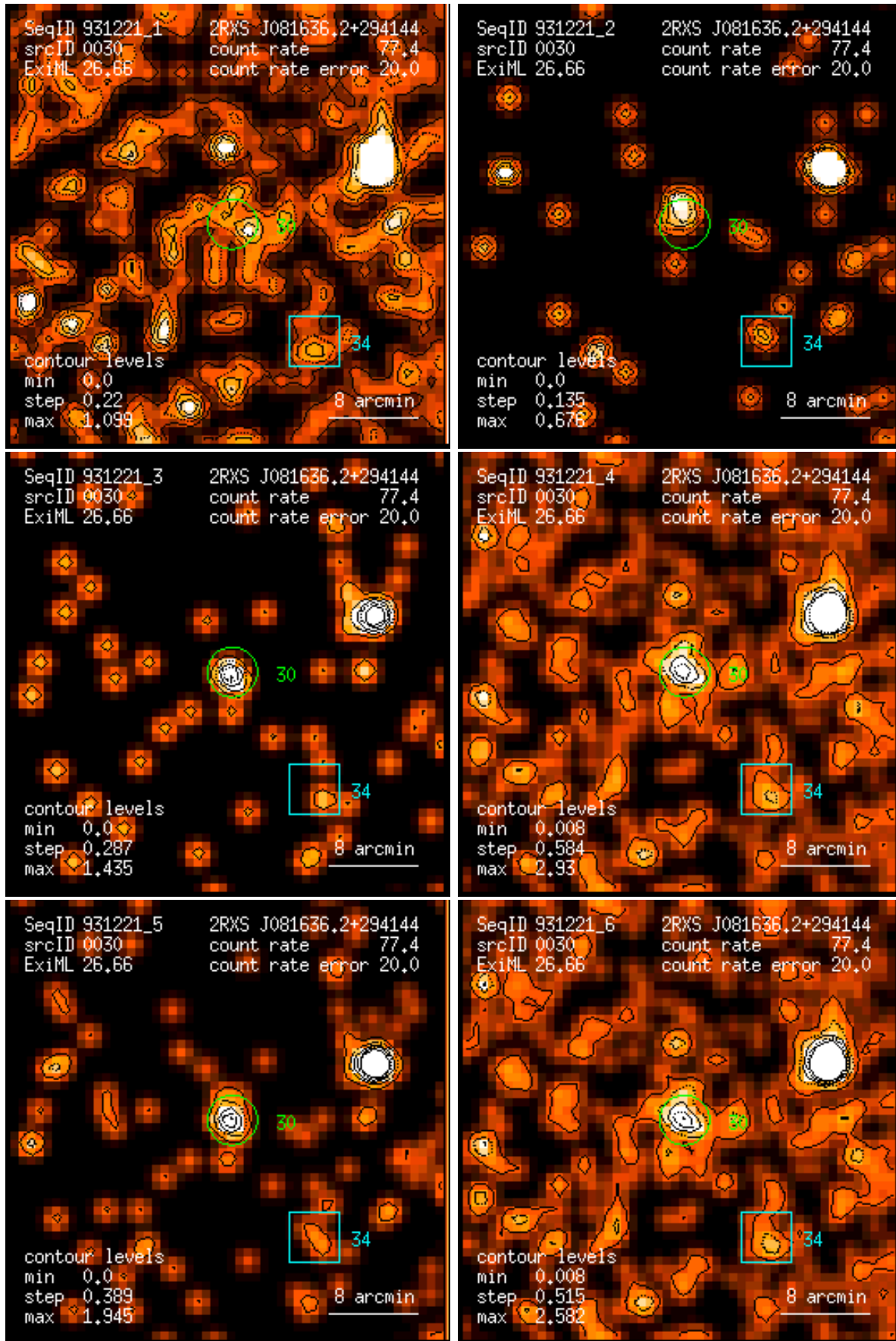
Figure 30: RASS 931221: detection 0030: band rate images, Gaussian filter: (1) PSPC channels 11 – 41, (2) 52 – 90, (3) 91 – 201, (4) 11 – 235, (5) 52 – 201, (6) 11 – 201. Broad band rates in counts/ks. Band rate contour levels in counts/ks/arcmin 2 .
