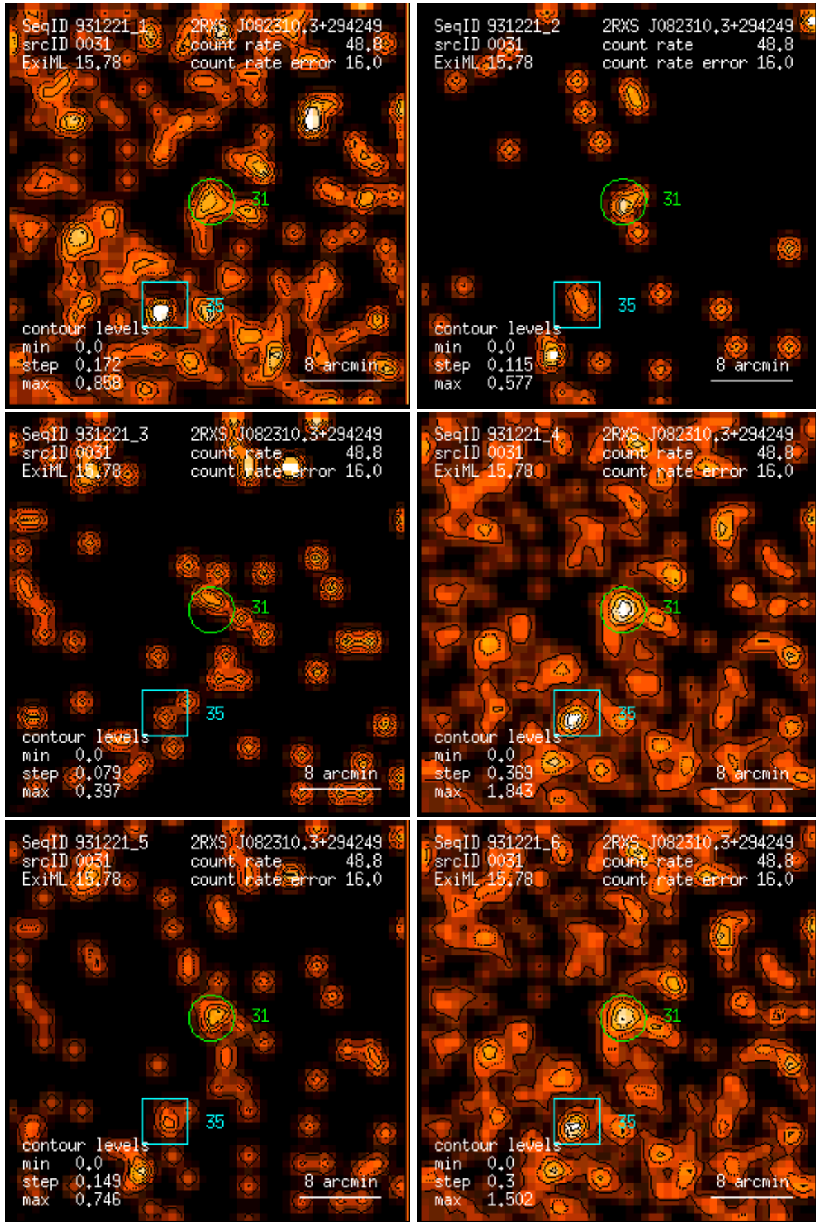
Figure 31: RASS 931221: detection 0031: band rate images, Gaussian filter: (1) PSPC channels 11 – 41, (2) 52 – 90, (3) 91 – 201, (4) 11 – 235, (5) 52 – 201, (6) 11 – 201. Broad band rates in counts/ks. Band rate contour levels in counts/ks/arcmin 2 .
