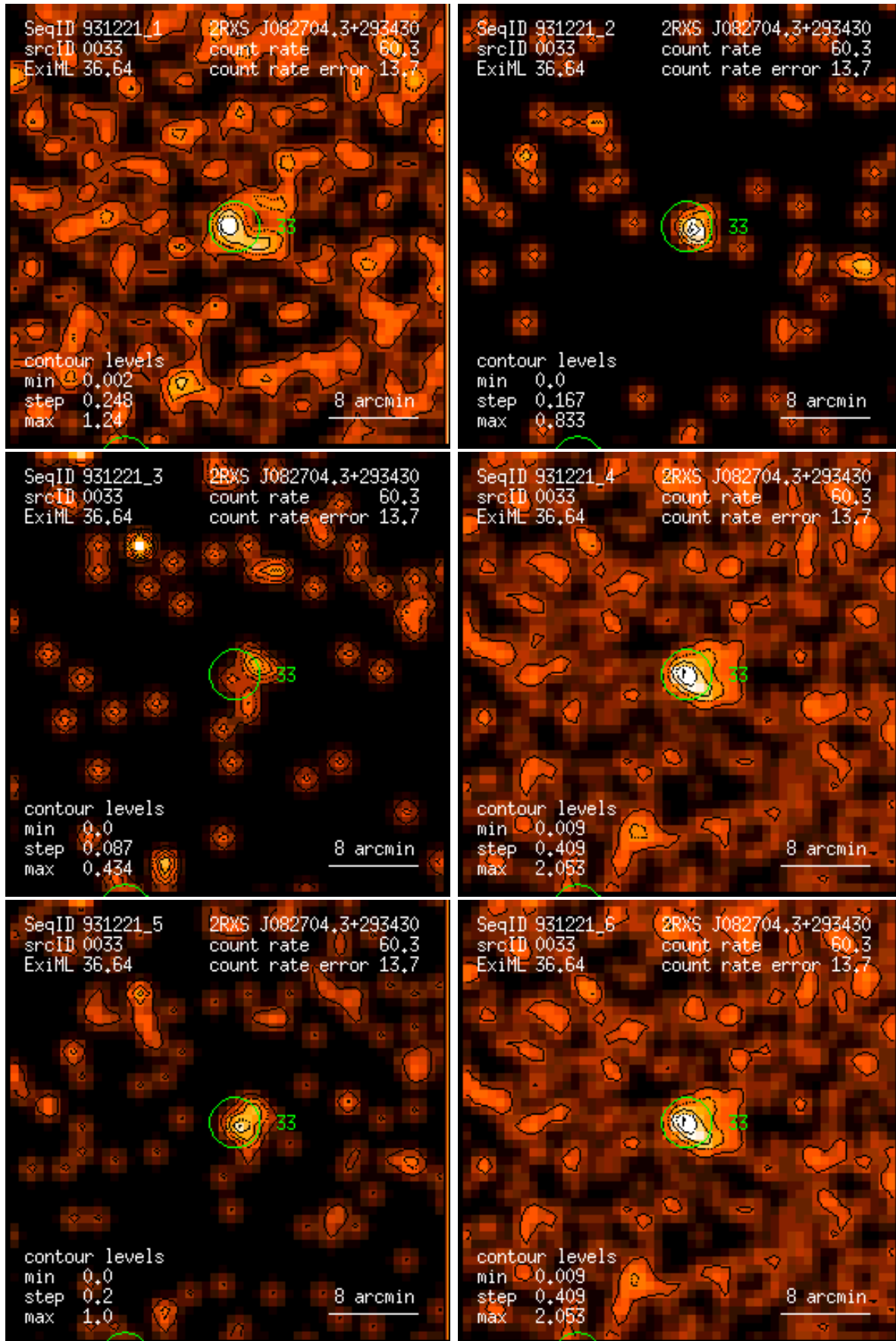
Figure 33: RASS 931221: detection 0033: band rate images, Gaussian filter: (1) PSPC channels 11 – 41, (2) 52 – 90, (3) 91 – 201, (4) 11 – 235, (5) 52 – 201, (6) 11 – 201. Broad band rates in counts/ks. Band rate contour levels in counts/ks/arcmin 2 .
