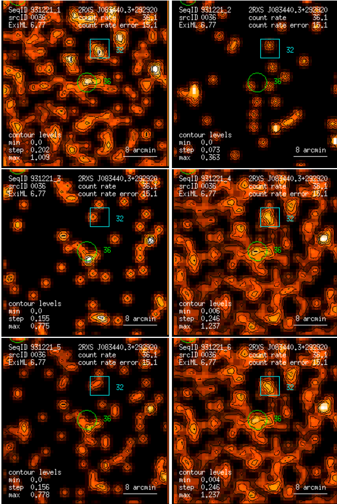
Figure 36: RASS 931221: detection 0036: band rate images, Gaussian filter: (1) PSPC channels 11 – 41, (2) 52 – 90, (3) 91 – 201, (4) 11 – 235, (5) 52 – 201, (6) 11 – 201. Broad band rates in counts/ks. Band rate contour levels in counts/ks/arcmin 2 .
