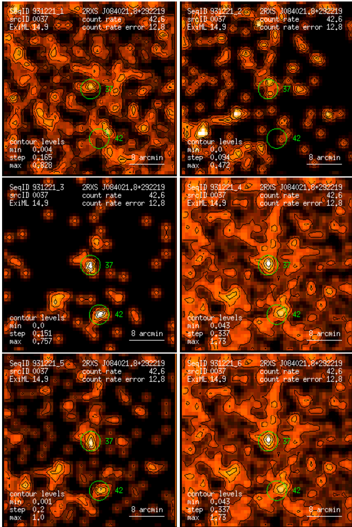
Figure 37: RASS 931221: detection 0037: band rate images, Gaussian filter: (1) PSPC channels 11 – 41, (2) 52 – 90, (3) 91 – 201, (4) 11 – 235, (5) 52 – 201, (6) 11 – 201. Broad band rates in counts/ks. Band rate contour levels in counts/ks/arcmin 2 .
