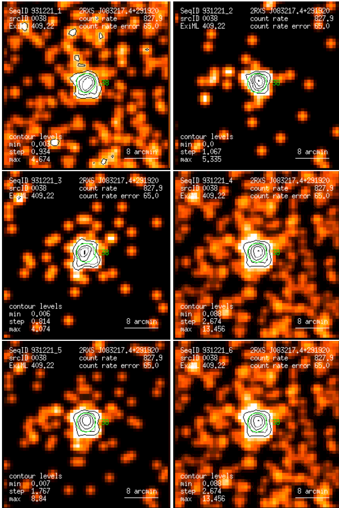
Figure 38: RASS 931221: detection 0038: band rate images, Gaussian filter: (1) PSPC channels 11 – 41, (2) 52 – 90, (3) 91 – 201, (4) 11 – 235, (5) 52 – 201, (6) 11 – 201. Broad band rates in counts/ks. Band rate contour levels in counts/ks/arcmin 2 .
