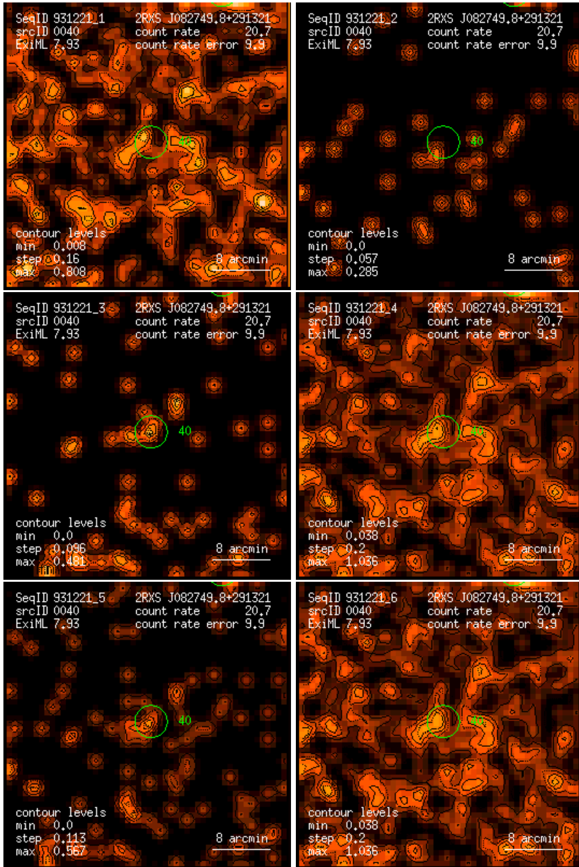
Figure 40: RASS 931221: detection 0040: band rate images, Gaussian filter: (1) PSPC channels 11 – 41, (2) 52 – 90, (3) 91 – 201, (4) 11 – 235, (5) 52 – 201, (6) 11 – 201. Broad band rates in counts/ks. Band rate contour levels in counts/ks/arcmin 2 .
