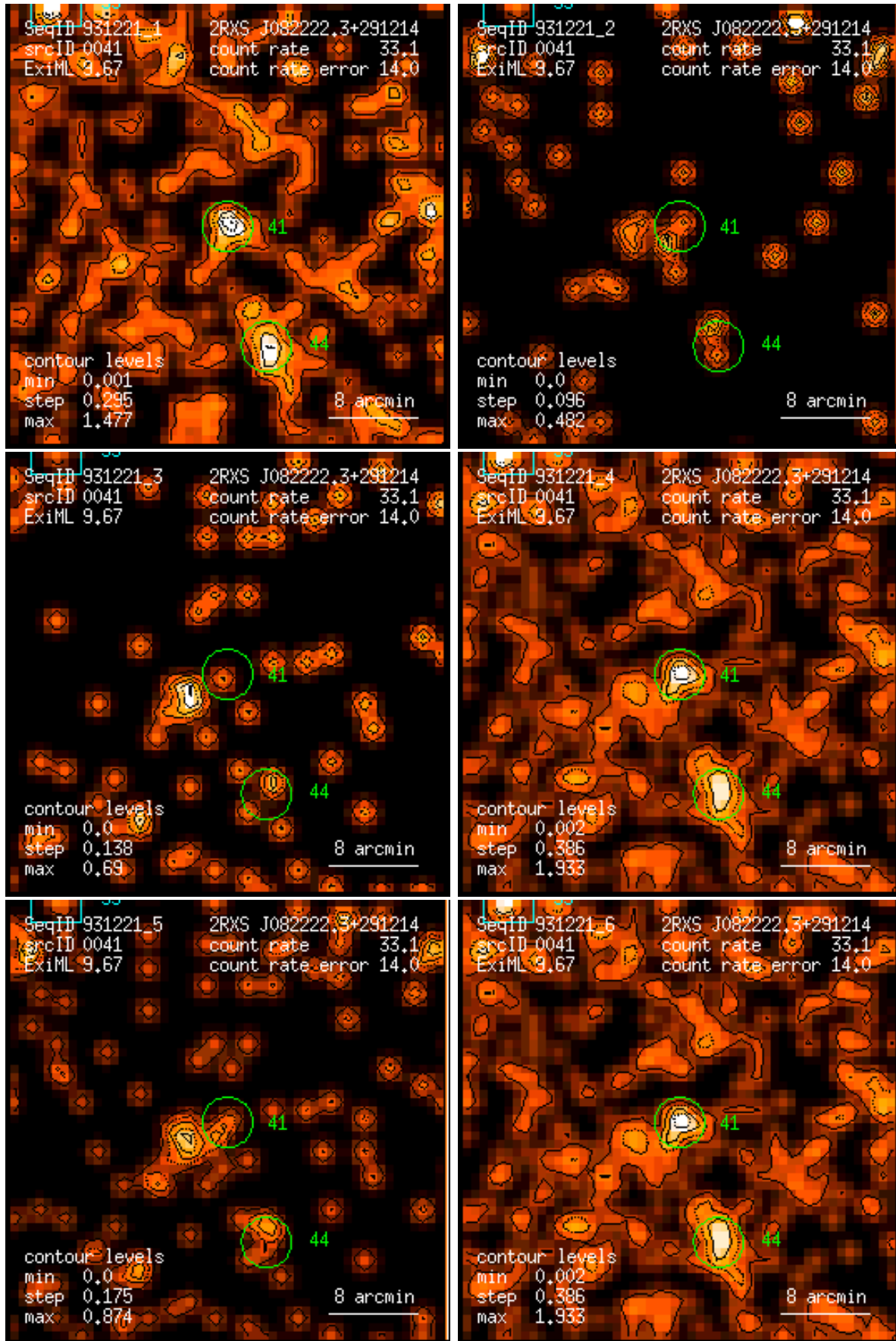
Figure 41: RASS 931221: detection 0041: band rate images, Gaussian filter: (1) PSPC channels 11 – 41, (2) 52 – 90, (3) 91 – 201, (4) 11 – 235, (5) 52 – 201, (6) 11 – 201. Broad band rates in counts/ks. Band rate contour levels in counts/ks/arcmin 2 .
