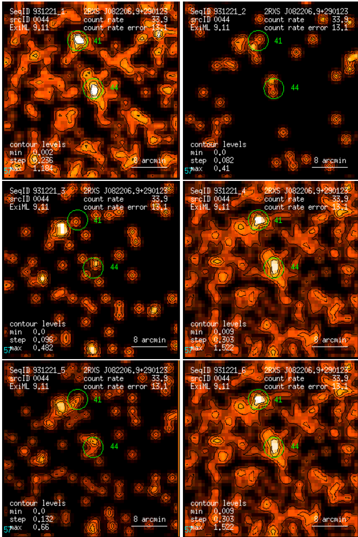
Figure 44: RASS 931221: detection 0044: band rate images, Gaussian filter: (1) PSPC channels 11 – 41, (2) 52 – 90, (3) 91 – 201, (4) 11 – 235, (5) 52 – 201, (6) 11 – 201. Broad band rates in counts/ks. Band rate contour levels in counts/ks/arcmin 2 .
