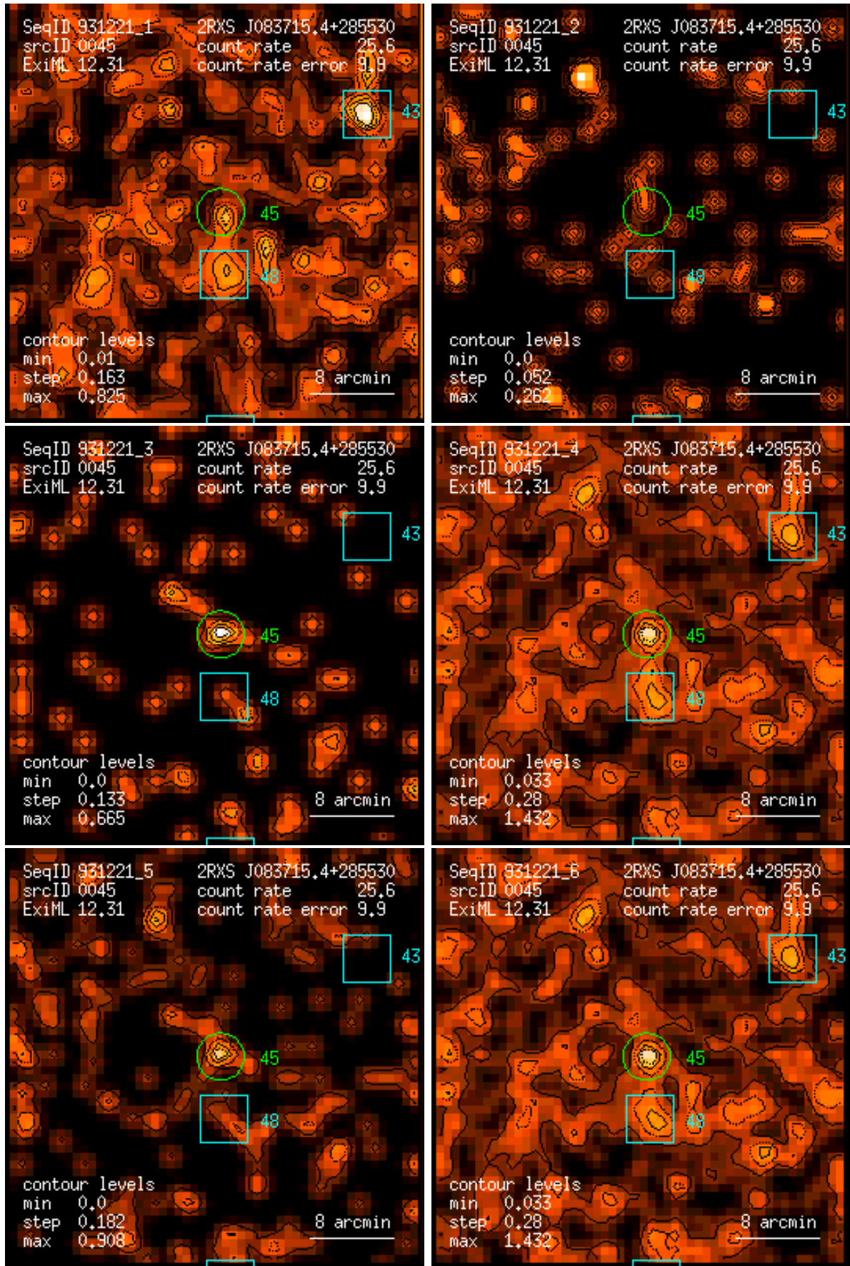
Figure 45: RASS 931221: detection 0045: band rate images, Gaussian filter: (1) PSPC channels 11 – 41, (2) 52 – 90, (3) 91 – 201, (4) 11 – 235, (5) 52 – 201, (6) 11 – 201. Broad band rates in counts/ks. Band rate contour levels in counts/ks/arcmin 2 .
