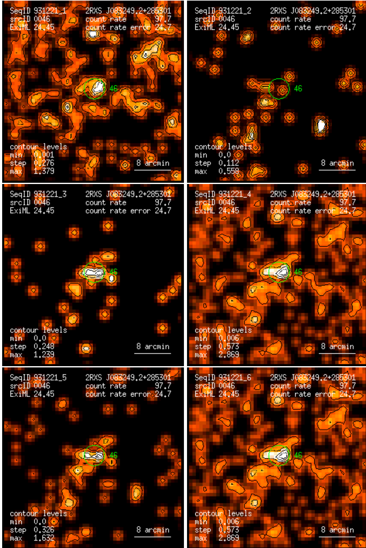
Figure 46: RASS 931221: detection 0046: band rate images, Gaussian filter: (1) PSPC channels 11 – 41, (2) 52 – 90, (3) 91 – 201, (4) 11 – 235, (5) 52 – 201, (6) 11 – 201. Broad band rates in counts/ks. Band rate contour levels in counts/ks/arcmin 2 .
