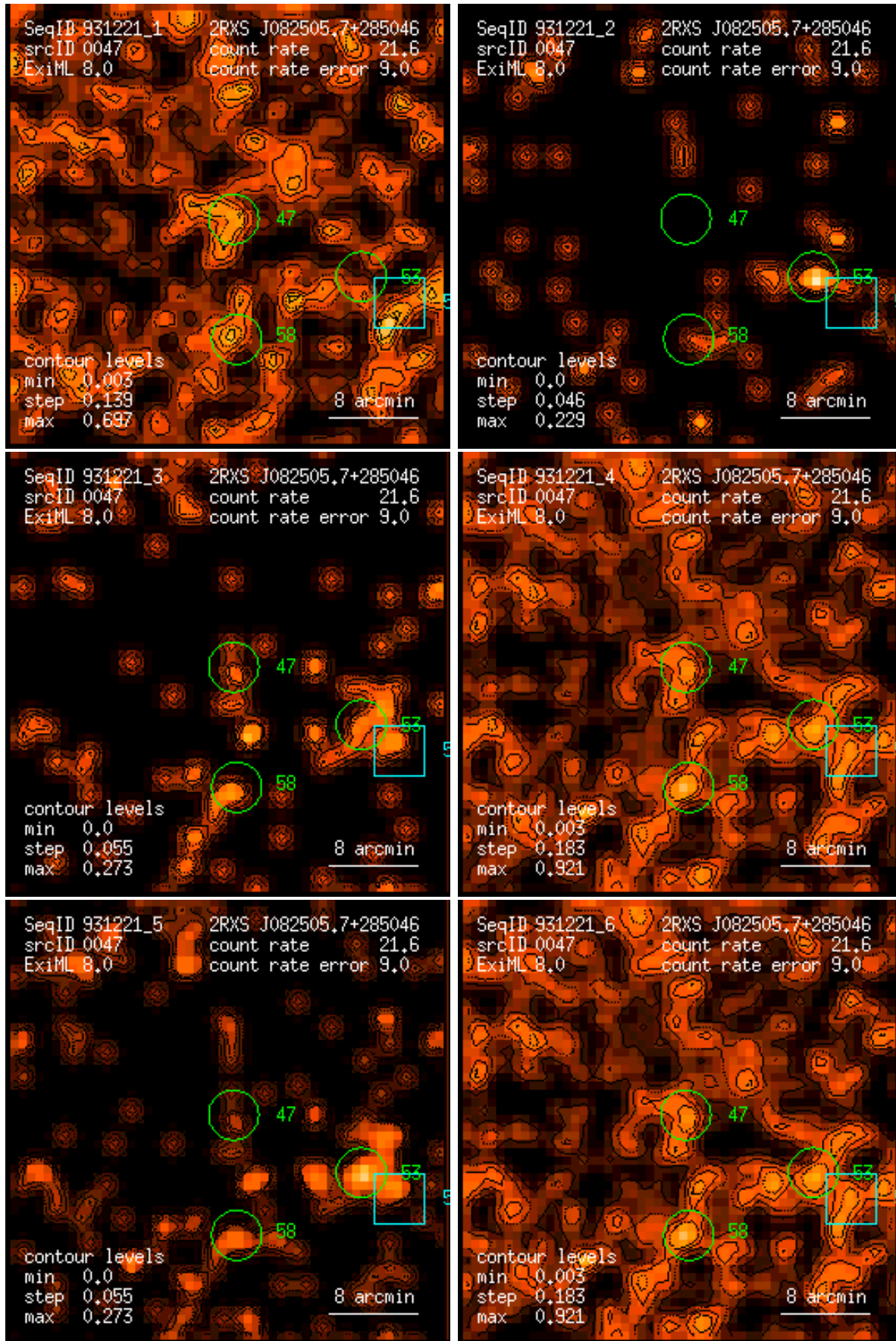
Figure 47: RASS 931221: detection 0047: band rate images, Gaussian filter: (1) PSPC channels 11 – 41, (2) 52 – 90, (3) 91 – 201, (4) 11 – 235, (5) 52 – 201, (6) 11 – 201. Broad band rates in counts/ks. Band rate contour levels in counts/ks/arcmin 2 .
