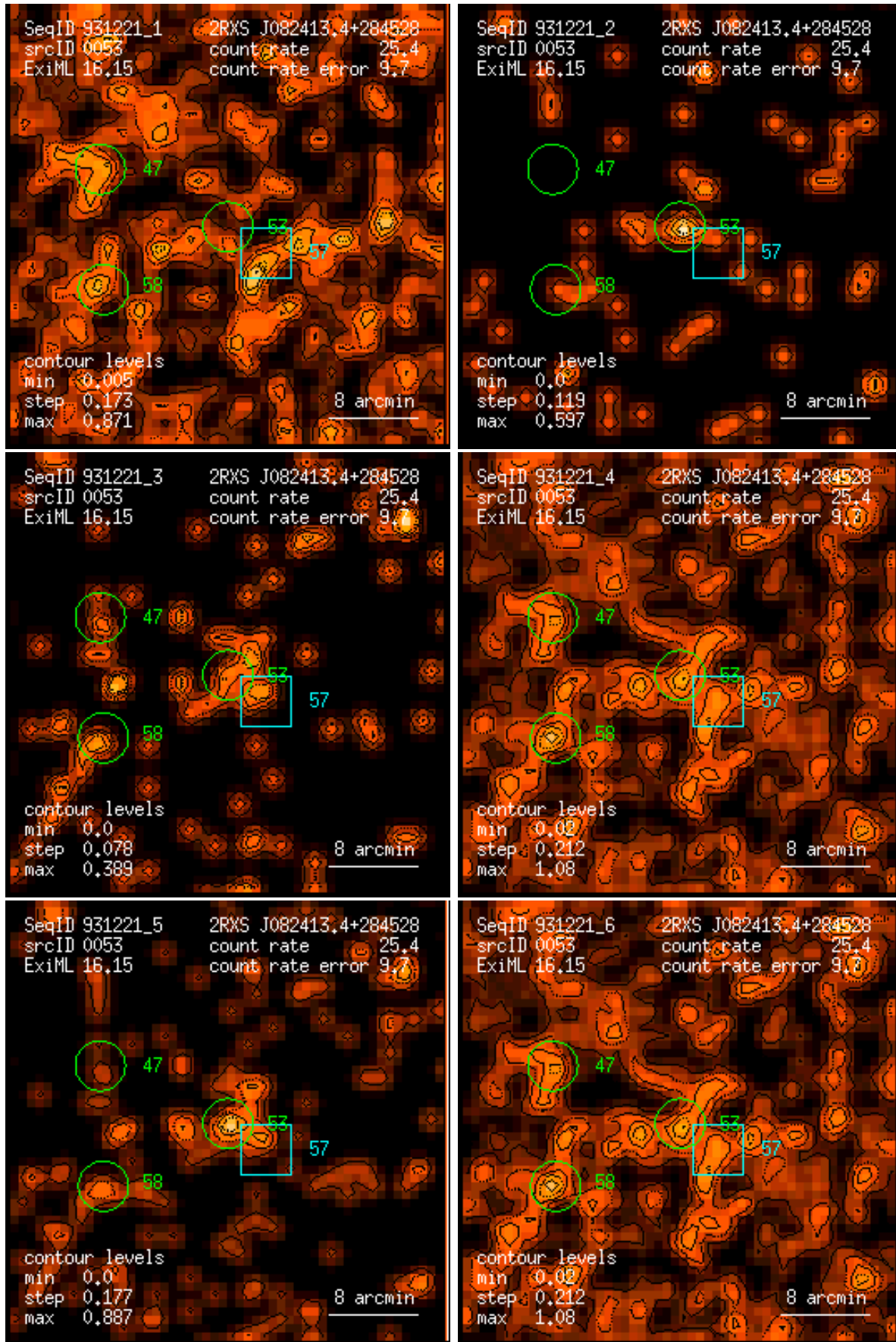
Figure 53: RASS 931221: detection 0053: band rate images, Gaussian filter: (1) PSPC channels 11 – 41, (2) 52 – 90, (3) 91 – 201, (4) 11 – 235, (5) 52 – 201, (6) 11 – 201. Broad band rates in counts/ks. Band rate contour levels in counts/ks/arcmin 2 .
