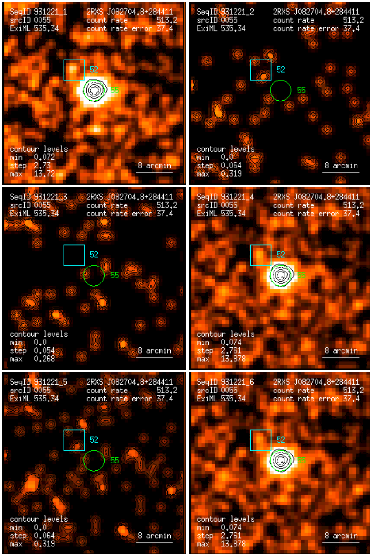
Figure 55: RASS 931221: detection 0055: band rate images, Gaussian filter: (1) PSPC channels 11 – 41, (2) 52 – 90, (3) 91 – 201, (4) 11 – 235, (5) 52 – 201, (6) 11 – 201. Broad band rates in counts/ks. Band rate contour levels in counts/ks/arcmin 2 .
