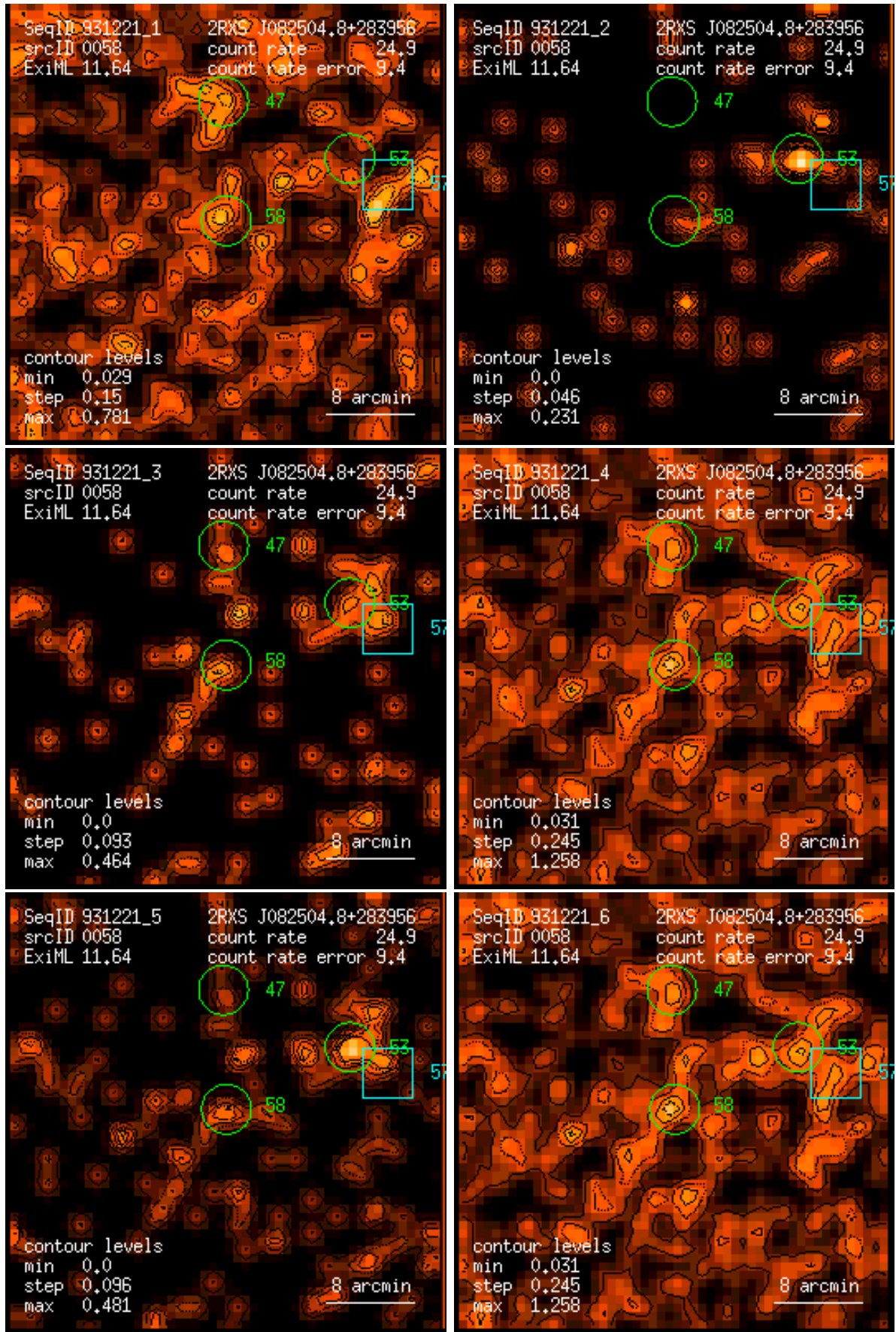
Figure 58: RASS 931221: detection 0058: band rate images, Gaussian filter: (1) PSPC channels 11 – 41, (2) 52 – 90, (3) 91 – 201, (4) 11 – 235, (5) 52 – 201, (6) 11 – 201. Broad band rates in counts/ks. Band rate contour levels in counts/ks/arcmin 2 .
