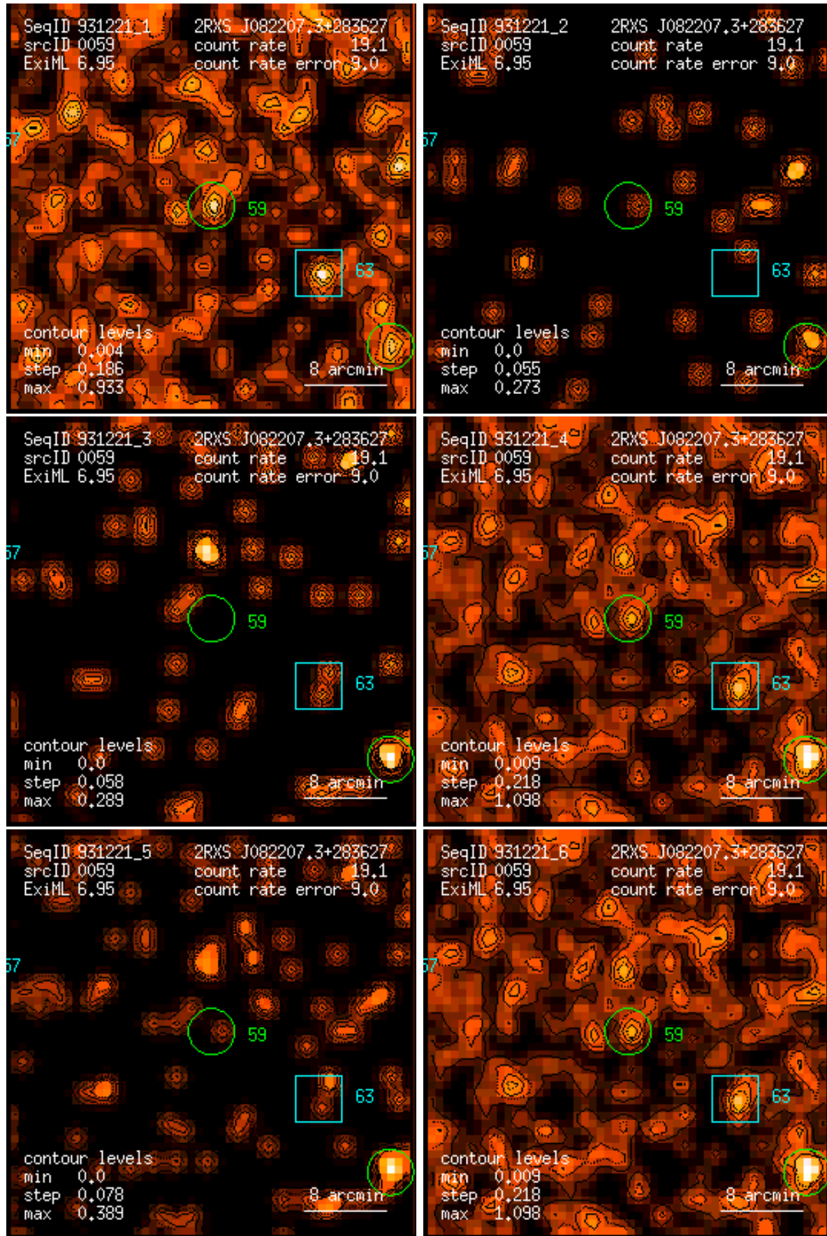
Figure 59: RASS 931221: detection 0059: band rate images, Gaussian filter: (1) PSPC channels 11 – 41, (2) 52 – 90, (3) 91 – 201, (4) 11 – 235, (5) 52 – 201, (6) 11 – 201. Broad band rates in counts/ks. Band rate contour levels in counts/ks/arcmin 2 .
