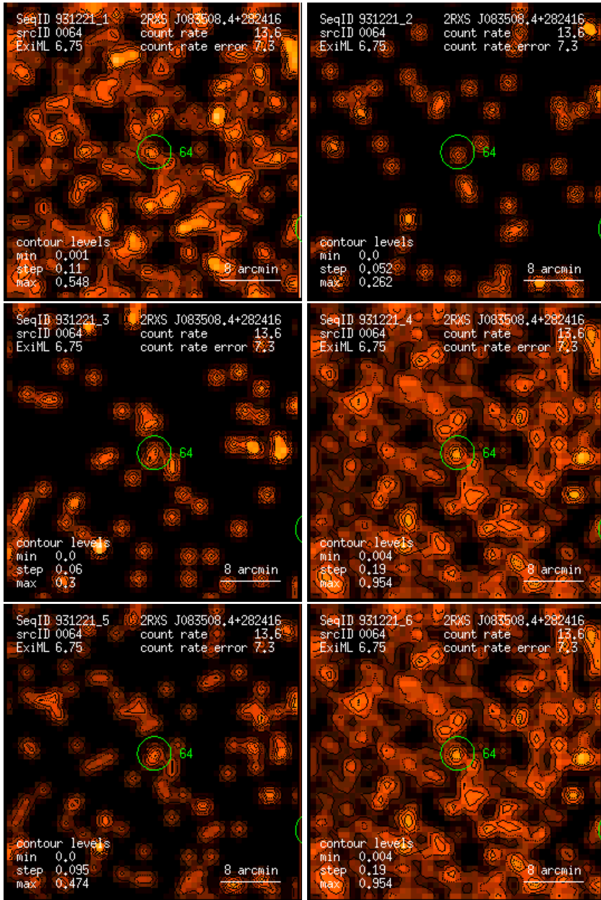
Figure 64: RASS 931221: detection 0064: band rate images, Gaussian filter: (1) PSPC channels 11 – 41, (2) 52 – 90, (3) 91 – 201, (4) 11 – 235, (5) 52 – 201, (6) 11 – 201. Broad band rates in counts/ks. Band rate contour levels in counts/ks/arcmin 2 .
