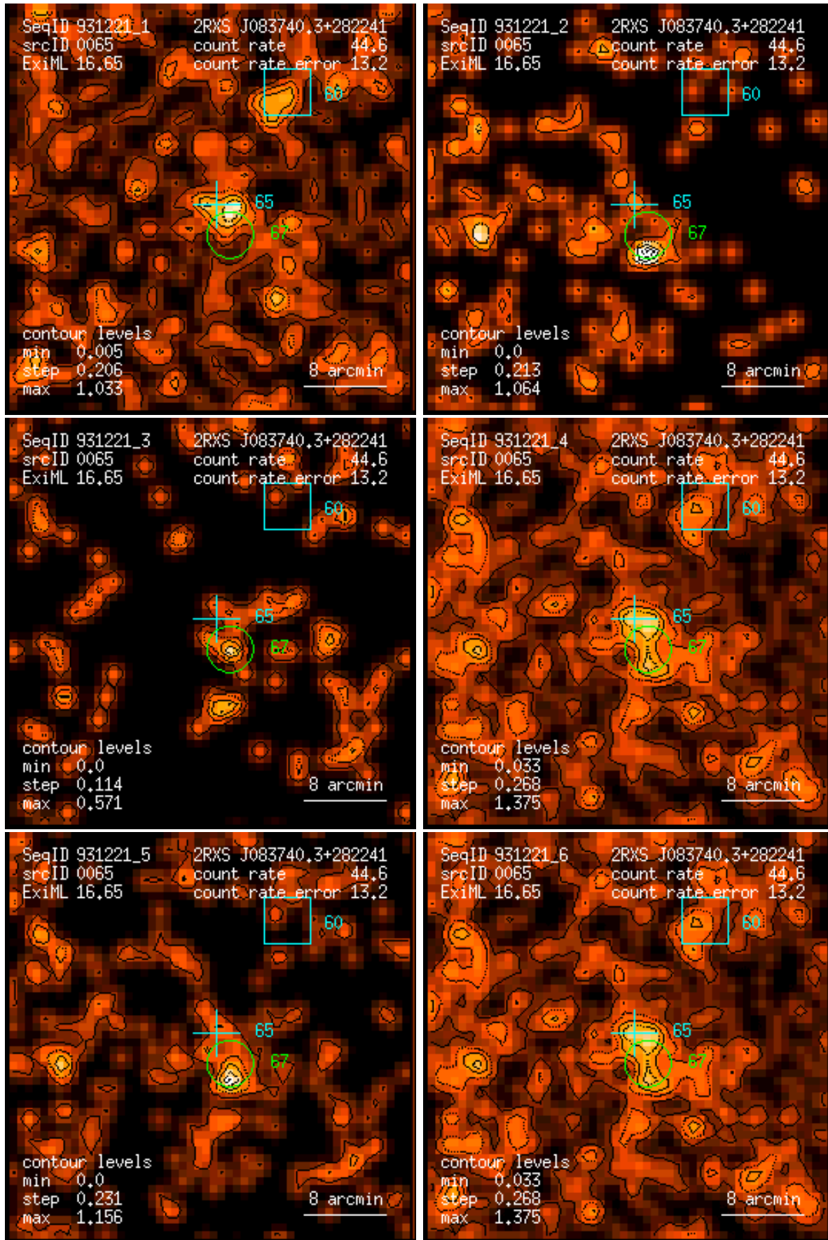
Figure 65: RASS 931221: detection 0065: band rate images, Gaussian filter: (1) PSPC channels 11 – 41, (2) 52 – 90, (3) 91 – 201, (4) 11 – 235, (5) 52 – 201, (6) 11 – 201. Broad band rates in counts/ks. Band rate contour levels in counts/ks/arcmin 2 .
