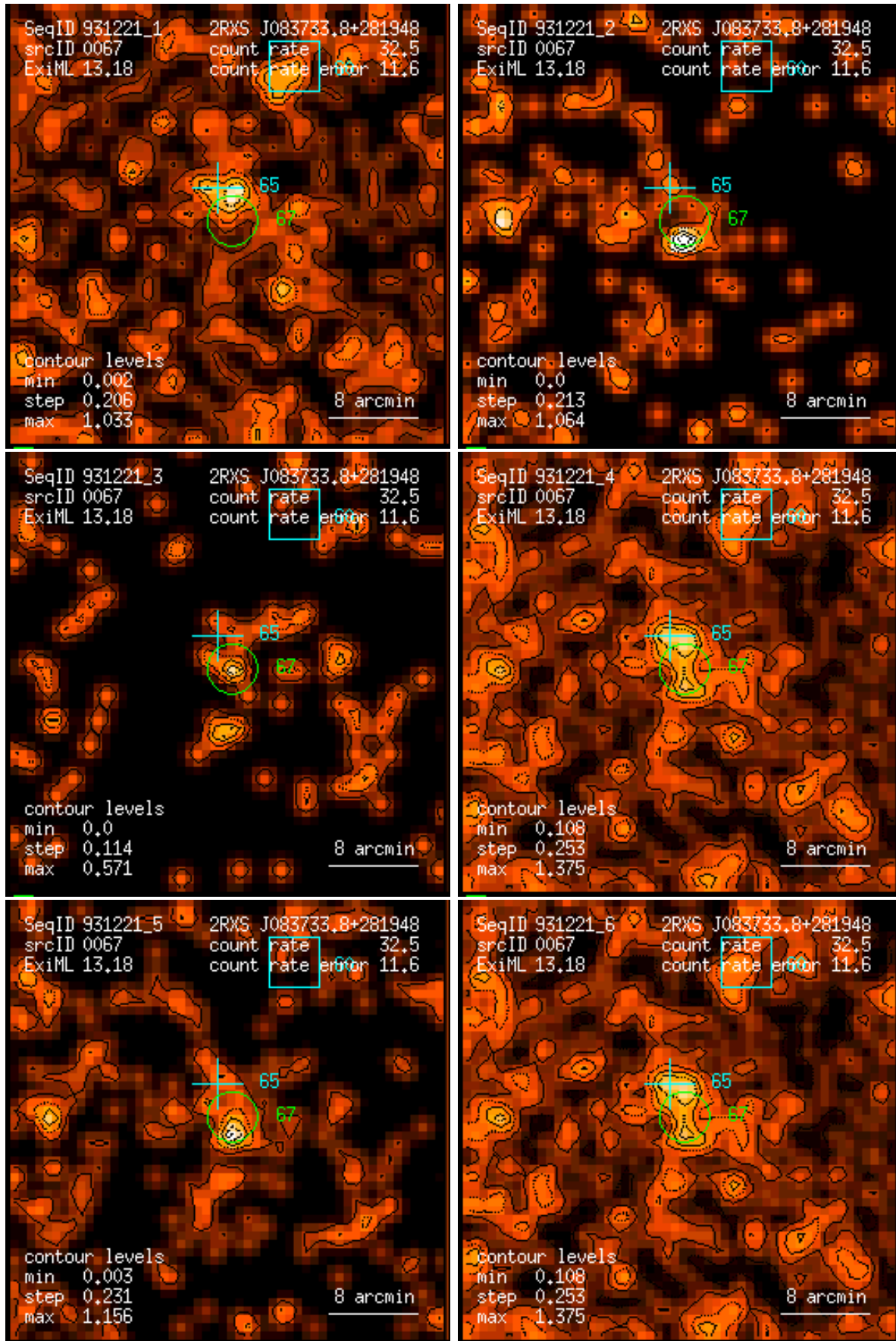
Figure 67: RASS 931221: detection 0067: band rate images, Gaussian filter: (1) PSPC channels 11 – 41, (2) 52 – 90, (3) 91 – 201, (4) 11 – 235, (5) 52 – 201, (6) 11 – 201. Broad band rates in counts/ks. Band rate contour levels in counts/ks/arcmin 2 .
