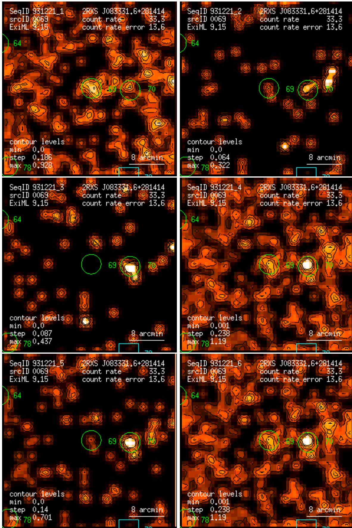
Figure 69: RASS 931221: detection 0069: band rate images, Gaussian filter: (1) PSPC channels 11 – 41, (2) 52 – 90, (3) 91 – 201, (4) 11 – 235, (5) 52 – 201, (6) 11 – 201. Broad band rates in counts/ks. Band rate contour levels in counts/ks/arcmin 2 .
