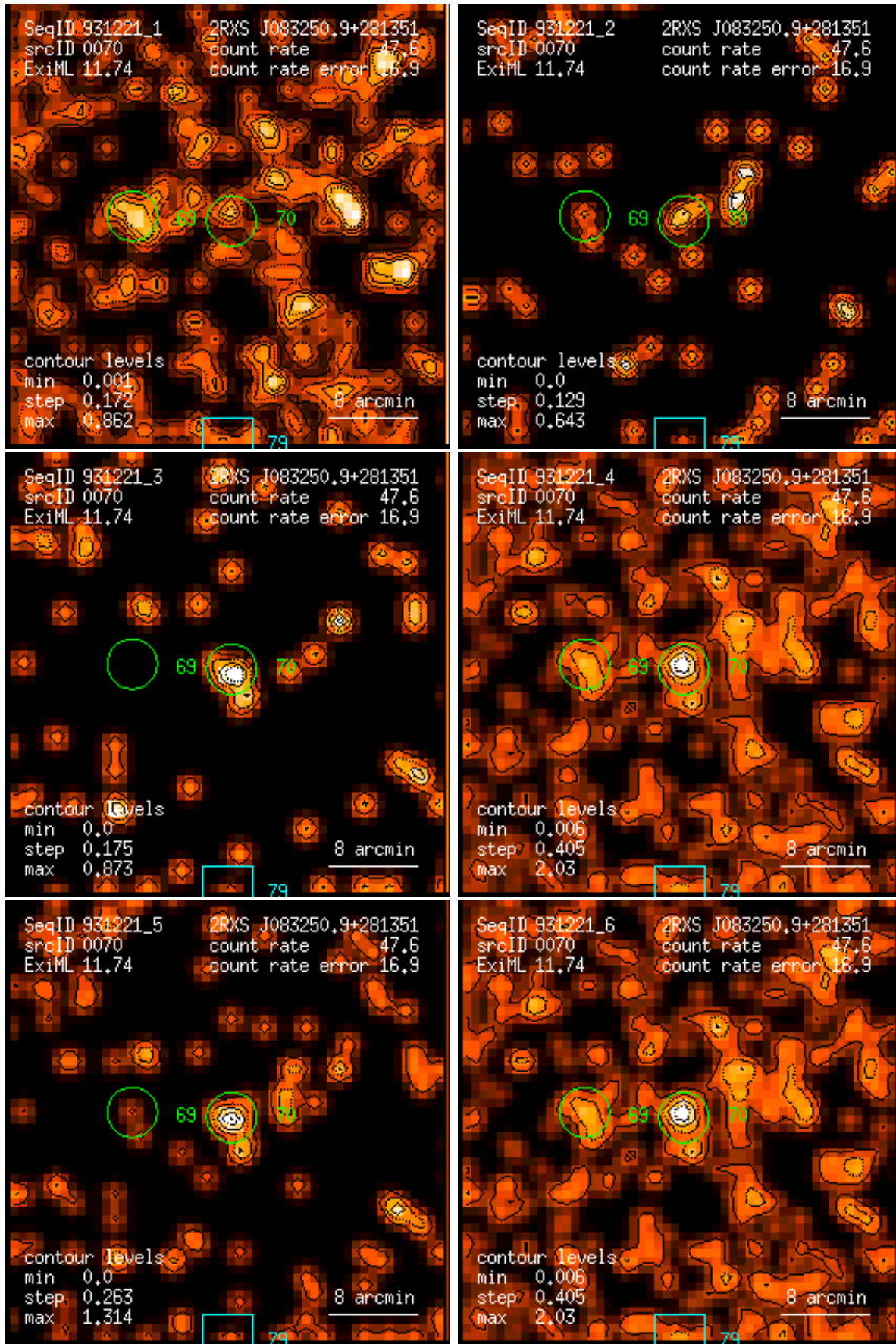
Figure 70: RASS 931221: detection 0070: band rate images, Gaussian filter: (1) PSPC channels 11 – 41, (2) 52 – 90, (3) 91 – 201, (4) 11 – 235, (5) 52 – 201, (6) 11 – 201. Broad band rates in counts/ks. Band rate contour levels in counts/ks/arcmin 2 .
