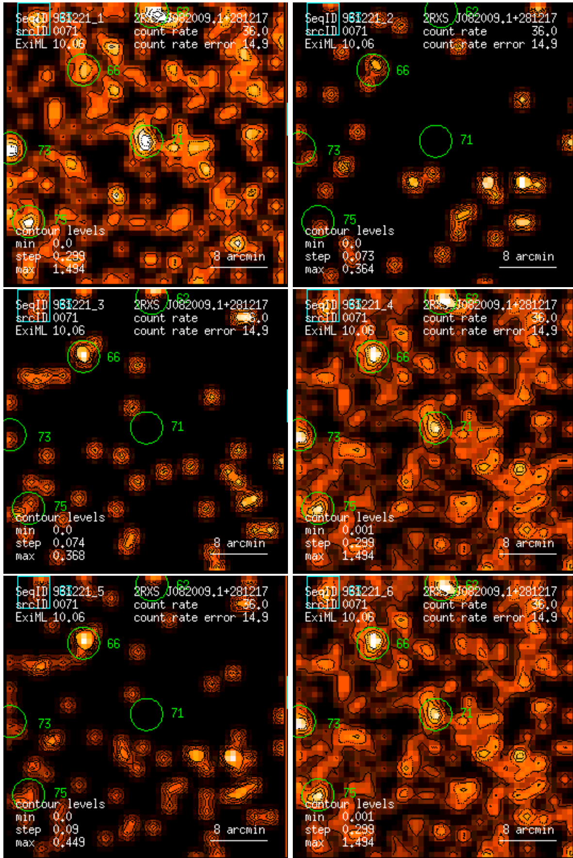
Figure 71: RASS 931221: detection 0071: band rate images, Gaussian filter: (1) PSPC channels 11 – 41, (2) 52 – 90, (3) 91 – 201, (4) 11 – 235, (5) 52 – 201, (6) 11 – 201. Broad band rates in counts/ks. Band rate contour levels in counts/ks/arcmin 2 .
