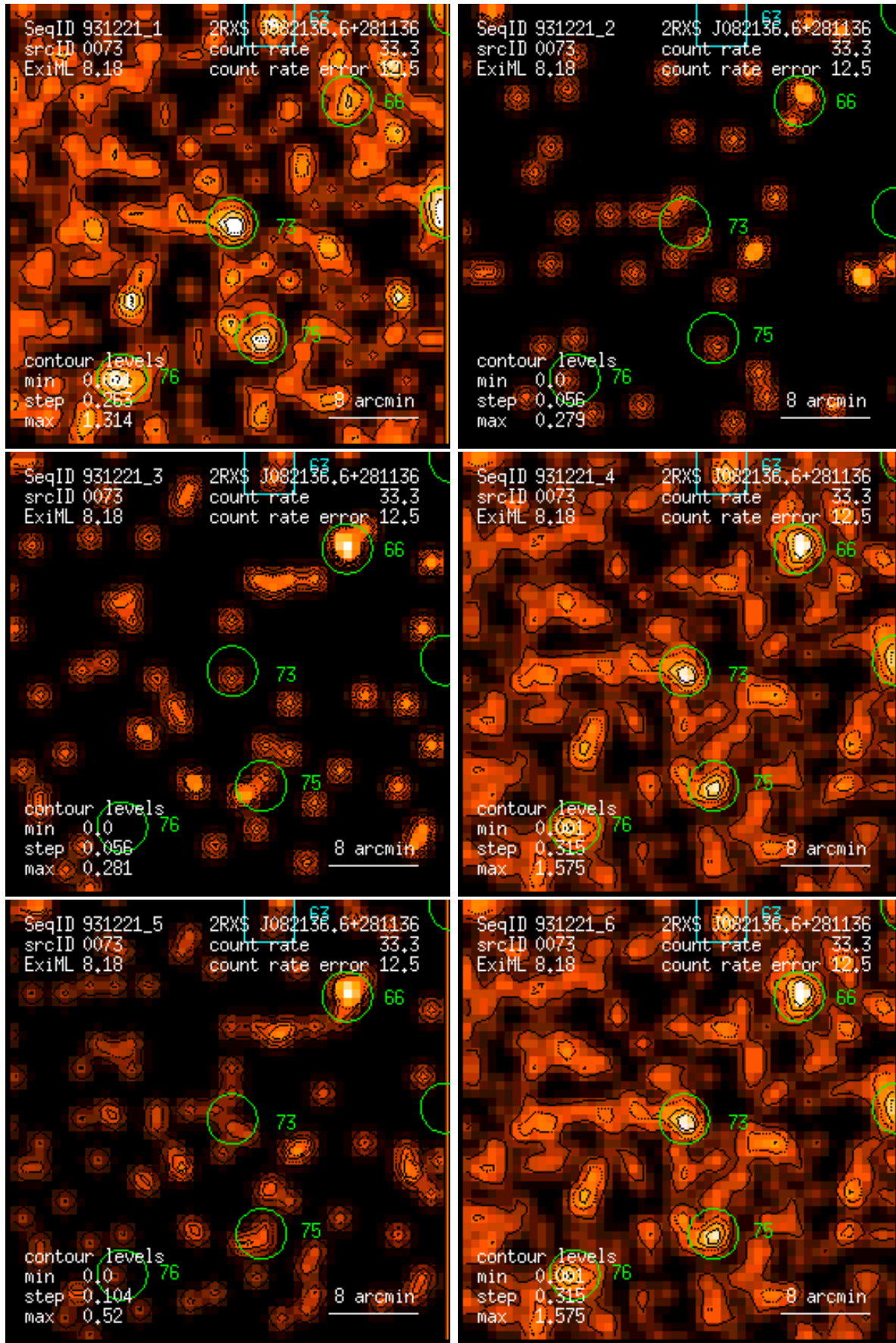
Figure 73: RASS 931221: detection 0073: band rate images, Gaussian filter: (1) PSPC channels 11 – 41, (2) 52 – 90, (3) 91 – 201, (4) 11 – 235, (5) 52 – 201, (6) 11 – 201. Broad band rates in counts/ks. Band rate contour levels in counts/ks/arcmin 2 .
