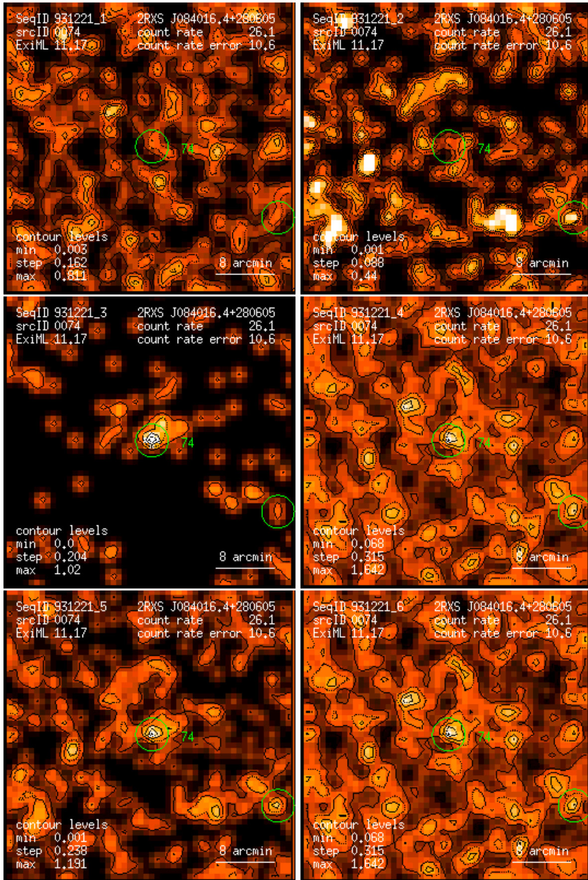
Figure 74: RASS 931221: detection 0074: band rate images, Gaussian filter: (1) PSPC channels 11 – 41, (2) 52 – 90, (3) 91 – 201, (4) 11 – 235, (5) 52 – 201, (6) 11 – 201. Broad band rates in counts/ks. Band rate contour levels in counts/ks/arcmin 2 .
