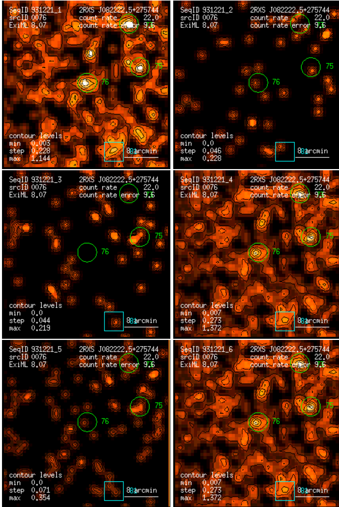
Figure 76: RASS 931221: detection 0076: band rate images, Gaussian filter: (1) PSPC channels 11 – 41, (2) 52 – 90, (3) 91 – 201, (4) 11 – 235, (5) 52 – 201, (6) 11 – 201. Broad band rates in counts/ks. Band rate contour levels in counts/ks/arcmin 2 .
