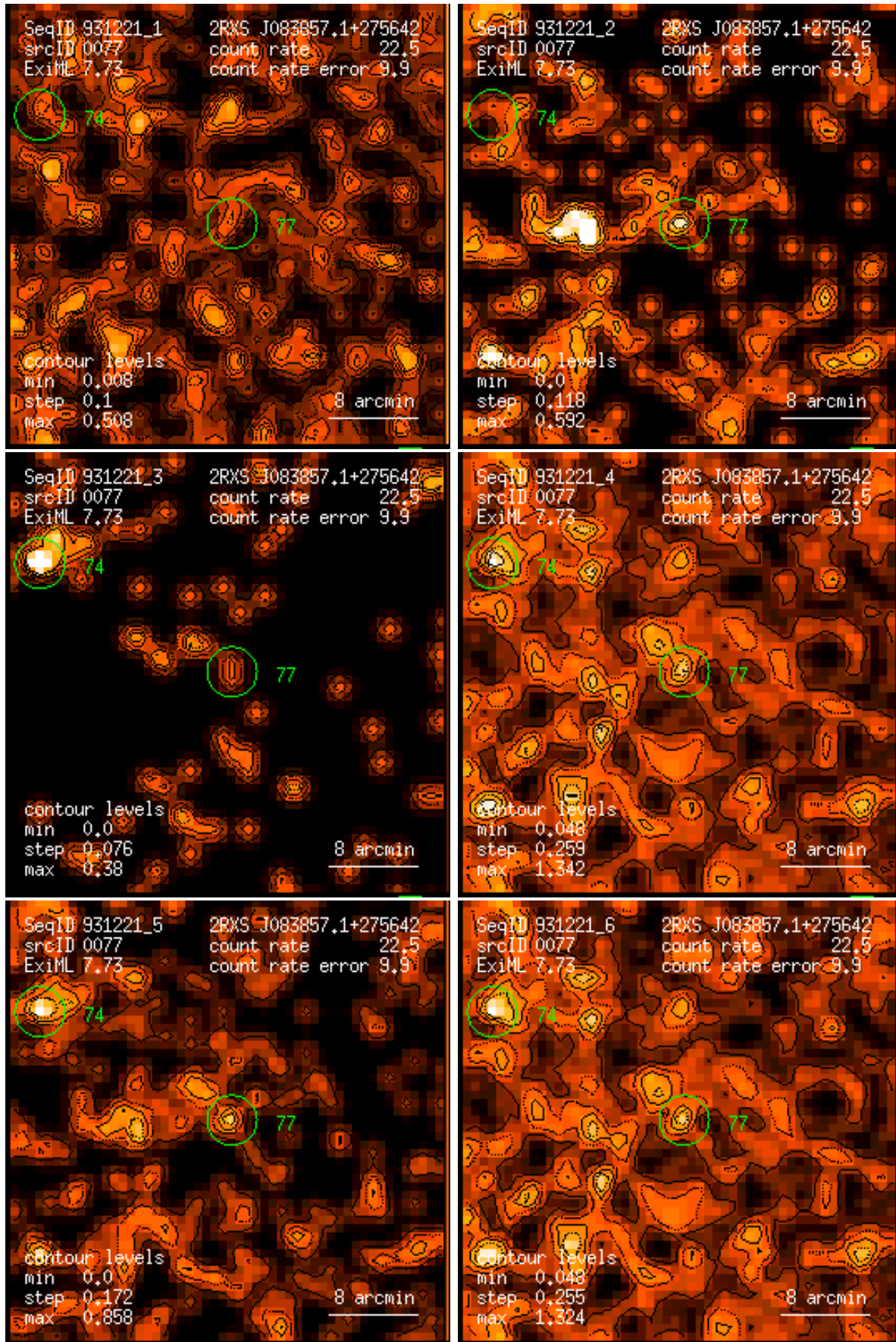
Figure 77: RASS 931221: detection 0077: band rate images, Gaussian filter: (1) PSPC channels 11 – 41, (2) 52 – 90, (3) 91 – 201, (4) 11 – 235, (5) 52 – 201, (6) 11 – 201. Broad band rates in counts/ks. Band rate contour levels in counts/ks/arcmin 2 .
