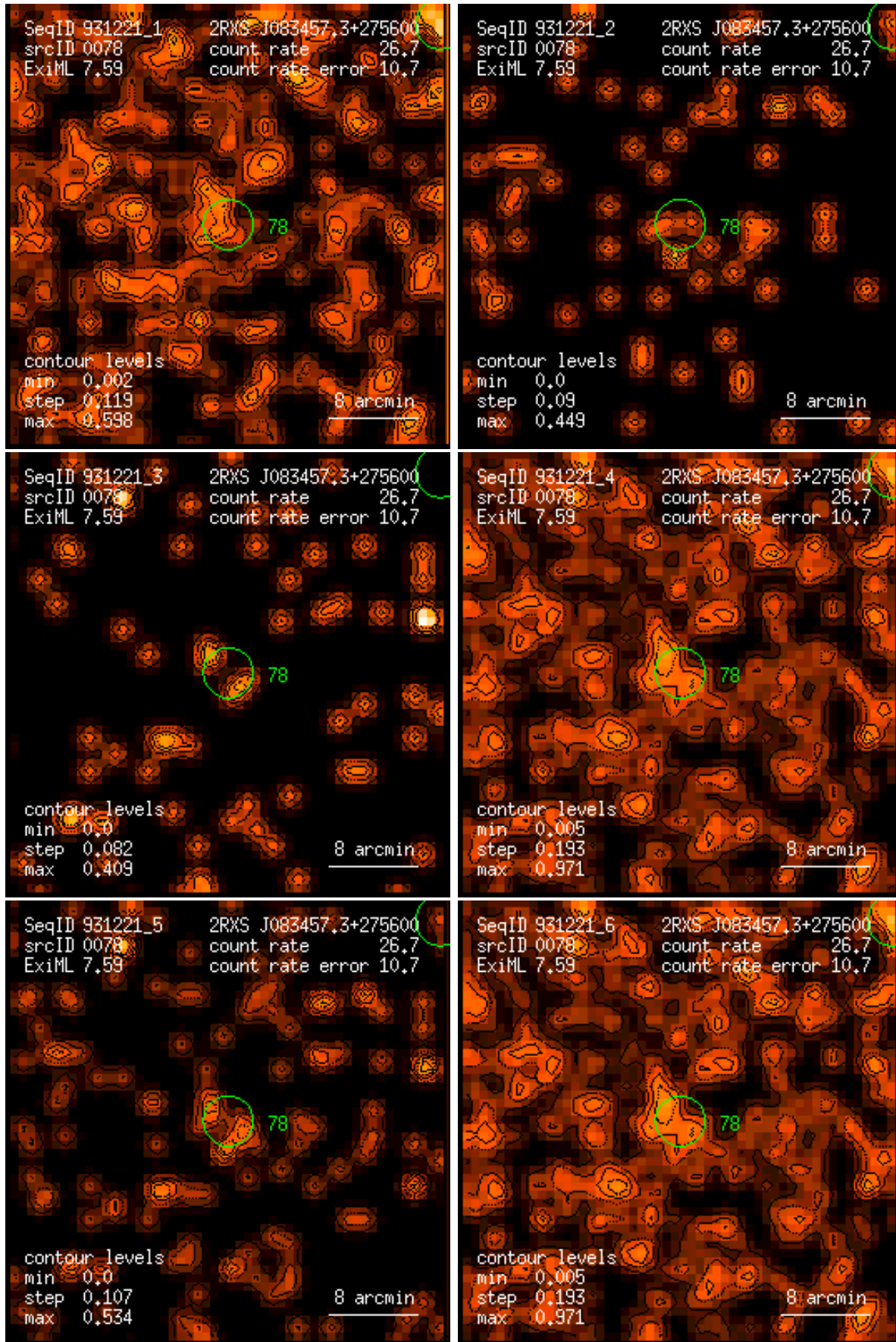
Figure 78: RASS 931221: detection 0078: band rate images, Gaussian filter: (1) PSPC channels 11 – 41, (2) 52 – 90, (3) 91 – 201, (4) 11 – 235, (5) 52 – 201, (6) 11 – 201. Broad band rates in counts/ks. Band rate contour levels in counts/ks/arcmin 2 .
