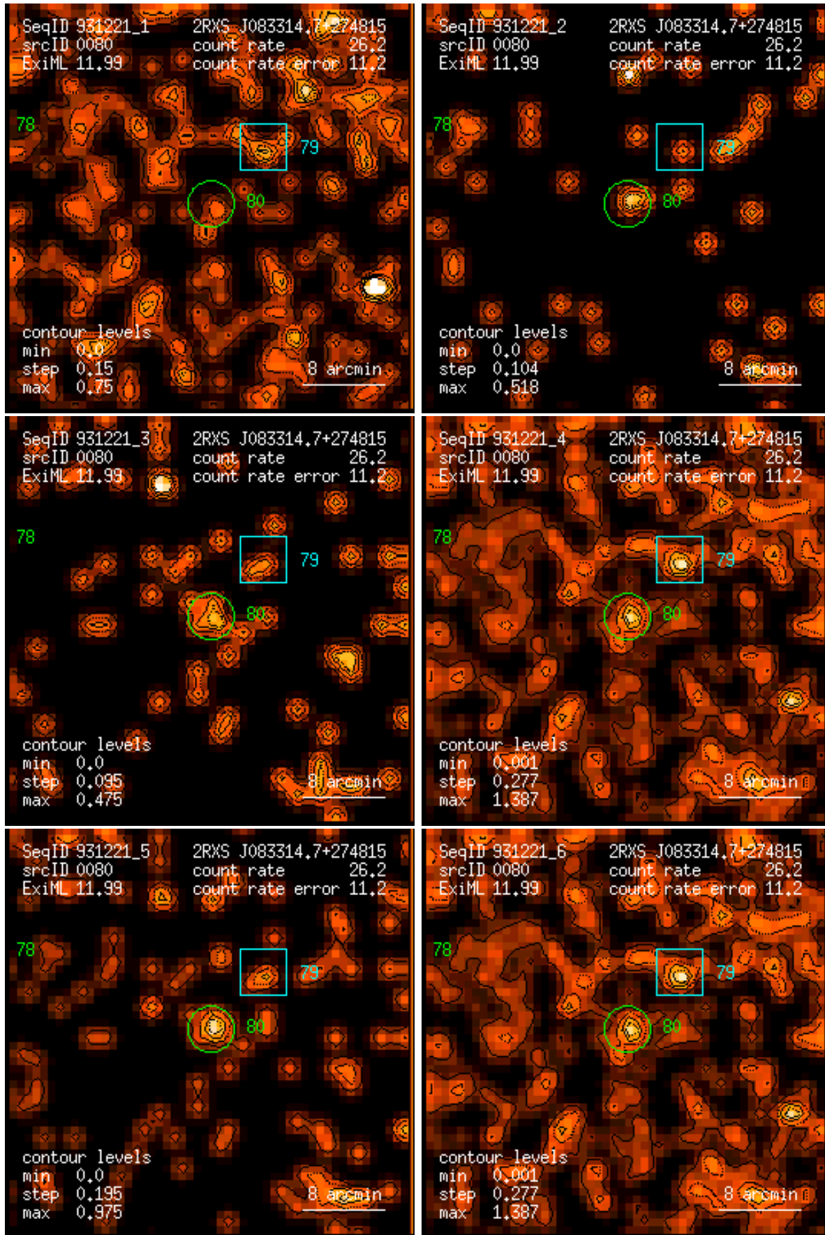
Figure 80: RASS 931221: detection 0080: band rate images, Gaussian filter: (1) PSPC channels 11 – 41, (2) 52 – 90, (3) 91 – 201, (4) 11 – 235, (5) 52 – 201, (6) 11 – 201. Broad band rates in counts/ks. Band rate contour levels in counts/ks/arcmin 2 .
