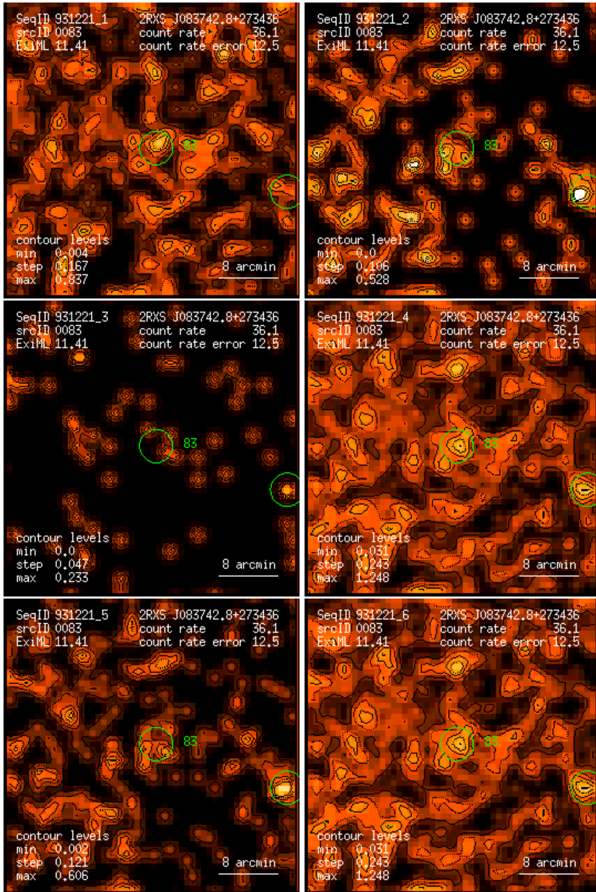
Figure 83: RASS 931221: detection 0083: band rate images, Gaussian filter: (1) PSPC channels 11 – 41, (2) 52 – 90, (3) 91 – 201, (4) 11 – 235, (5) 52 – 201, (6) 11 – 201. Broad band rates in counts/ks. Band rate contour levels in counts/ks/arcmin 2 .
