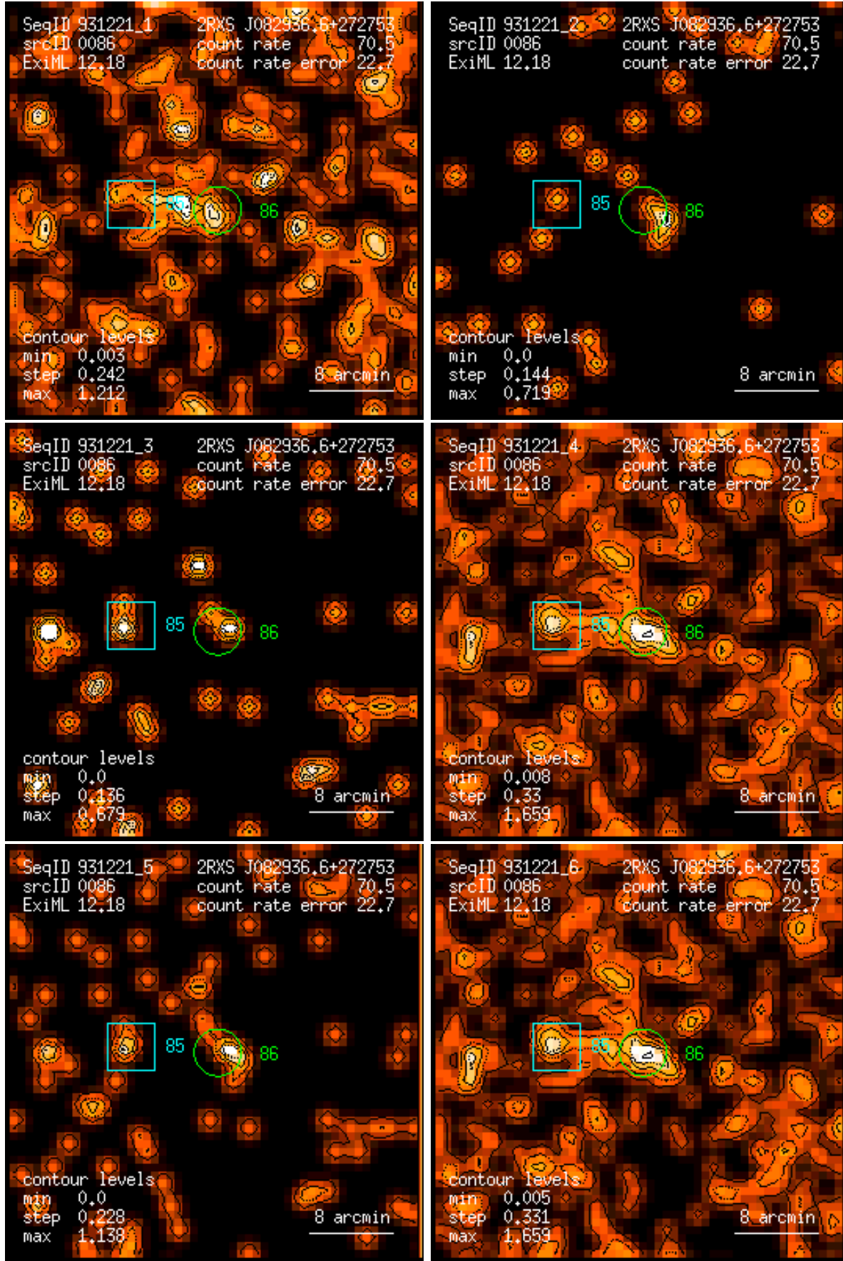
Figure 86: RASS 931221: detection 0086: band rate images, Gaussian filter: (1) PSPC channels 11 – 41, (2) 52 – 90, (3) 91 – 201, (4) 11 – 235, (5) 52 – 201, (6) 11 – 201. Broad band rates in counts/ks. Band rate contour levels in counts/ks/arcmin 2 .
