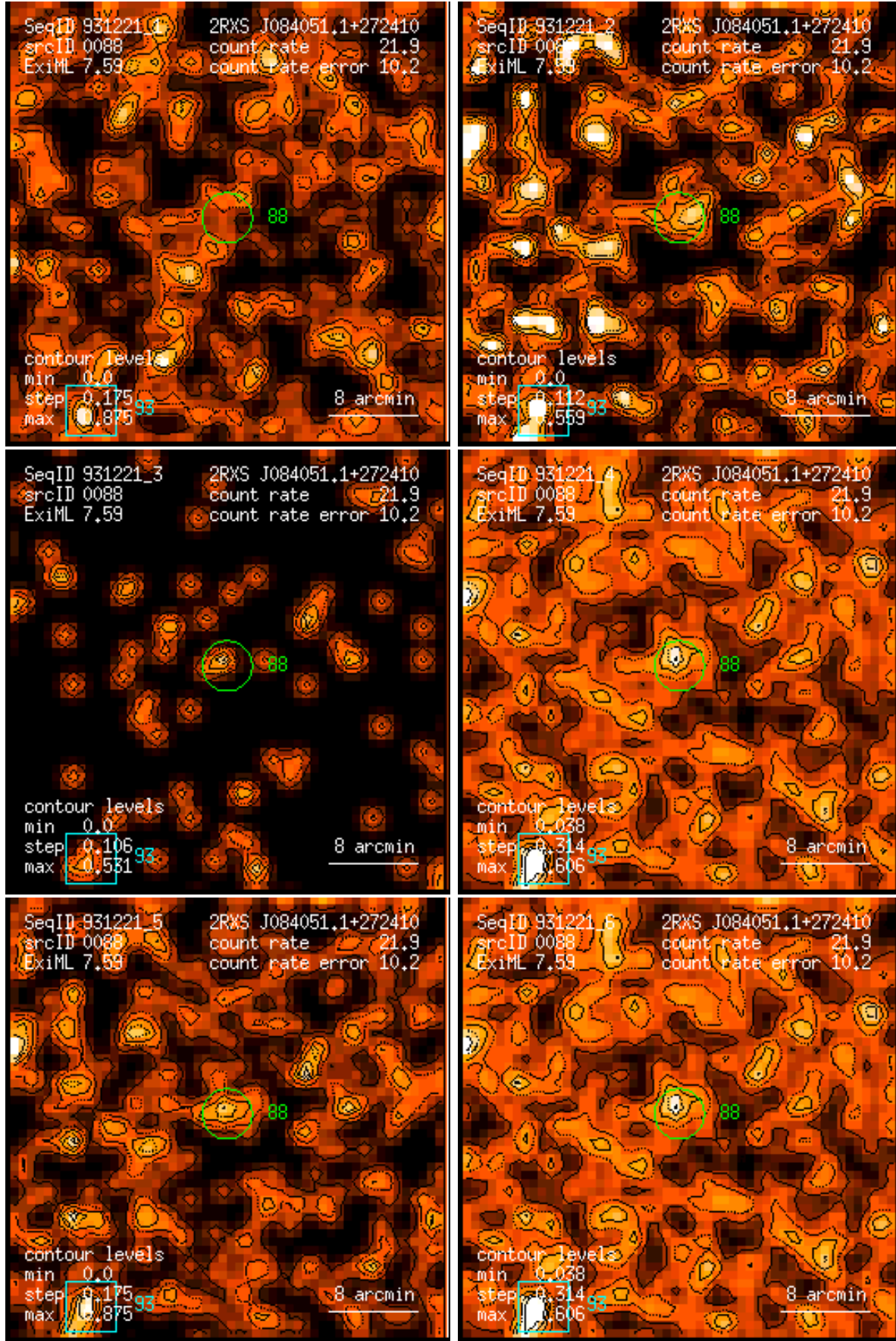
Figure 88: RASS 931221: detection 0088: band rate images, Gaussian filter: (1) PSPC channels 11 – 41, (2) 52 – 90, (3) 91 – 201, (4) 11 – 235, (5) 52 – 201, (6) 11 – 201. Broad band rates in counts/ks. Band rate contour levels in counts/ks/arcmin 2 .
