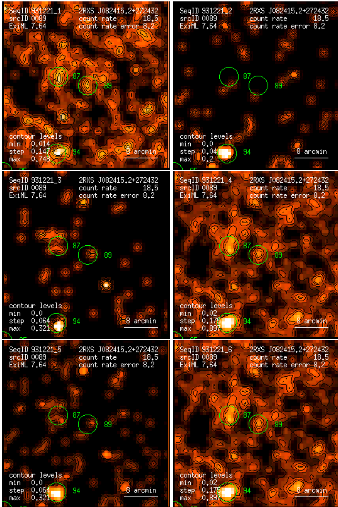
Figure 89: RASS 931221: detection 0089: band rate images, Gaussian filter: (1) PSPC channels 11 – 41, (2) 52 – 90, (3) 91 – 201, (4) 11 – 235, (5) 52 – 201, (6) 11 – 201. Broad band rates in counts/ks. Band rate contour levels in counts/ks/arcmin 2 .
