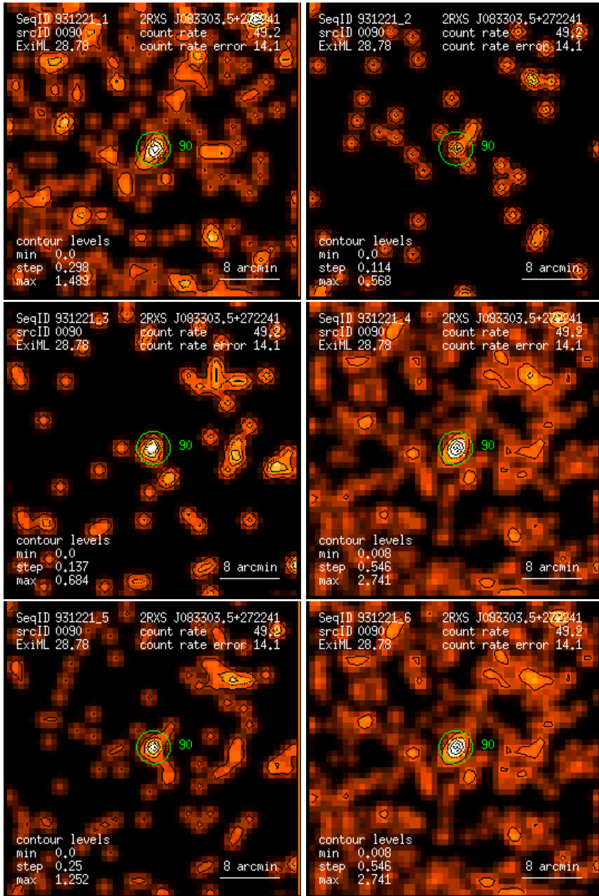
Figure 90: RASS 931221: detection 0090: band rate images, Gaussian filter: (1) PSPC channels 11 – 41, (2) 52 – 90, (3) 91 – 201, (4) 11 – 235, (5) 52 – 201, (6) 11 – 201. Broad band rates in counts/ks. Band rate contour levels in counts/ks/arcmin 2 .
