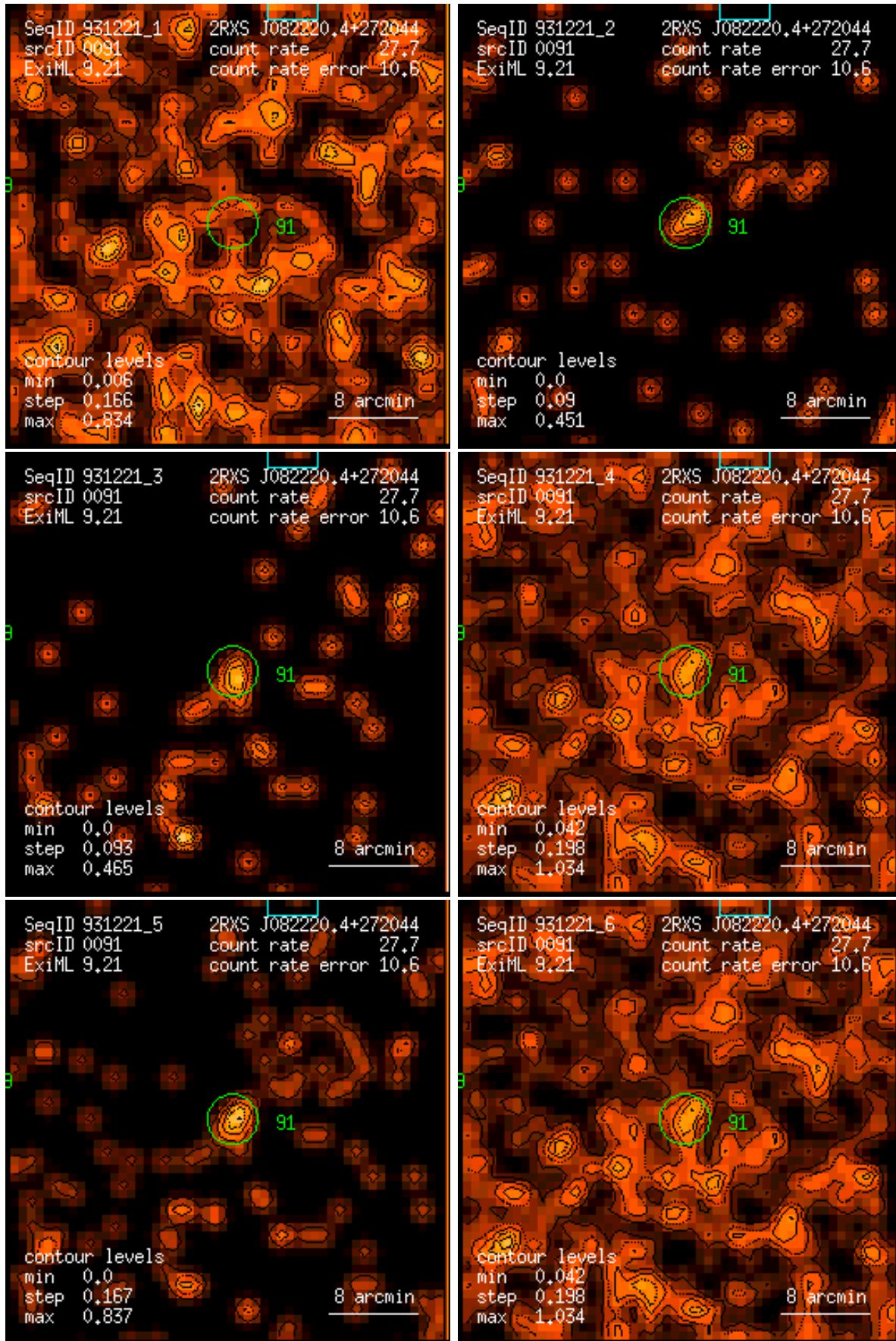
Figure 91: RASS 931221: detection 0091: band rate images, Gaussian filter: (1) PSPC channels 11 – 41, (2) 52 – 90, (3) 91 – 201, (4) 11 – 235, (5) 52 – 201, (6) 11 – 201. Broad band rates in counts/ks. Band rate contour levels in counts/ks/arcmin 2 .
