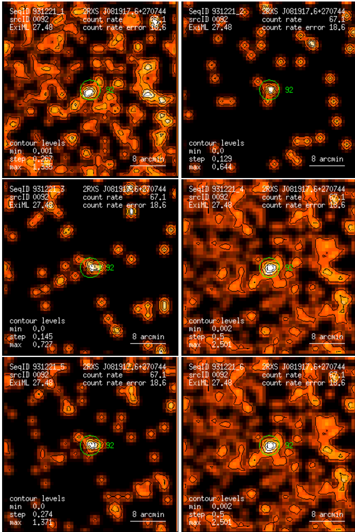
Figure 92: RASS 931221: detection 0092: band rate images, Gaussian filter: (1) PSPC channels 11 – 41, (2) 52 – 90, (3) 91 – 201, (4) 11 – 235, (5) 52 – 201, (6) 11 – 201. Broad band rates in counts/ks. Band rate contour levels in counts/ks/arcmin 2 .
