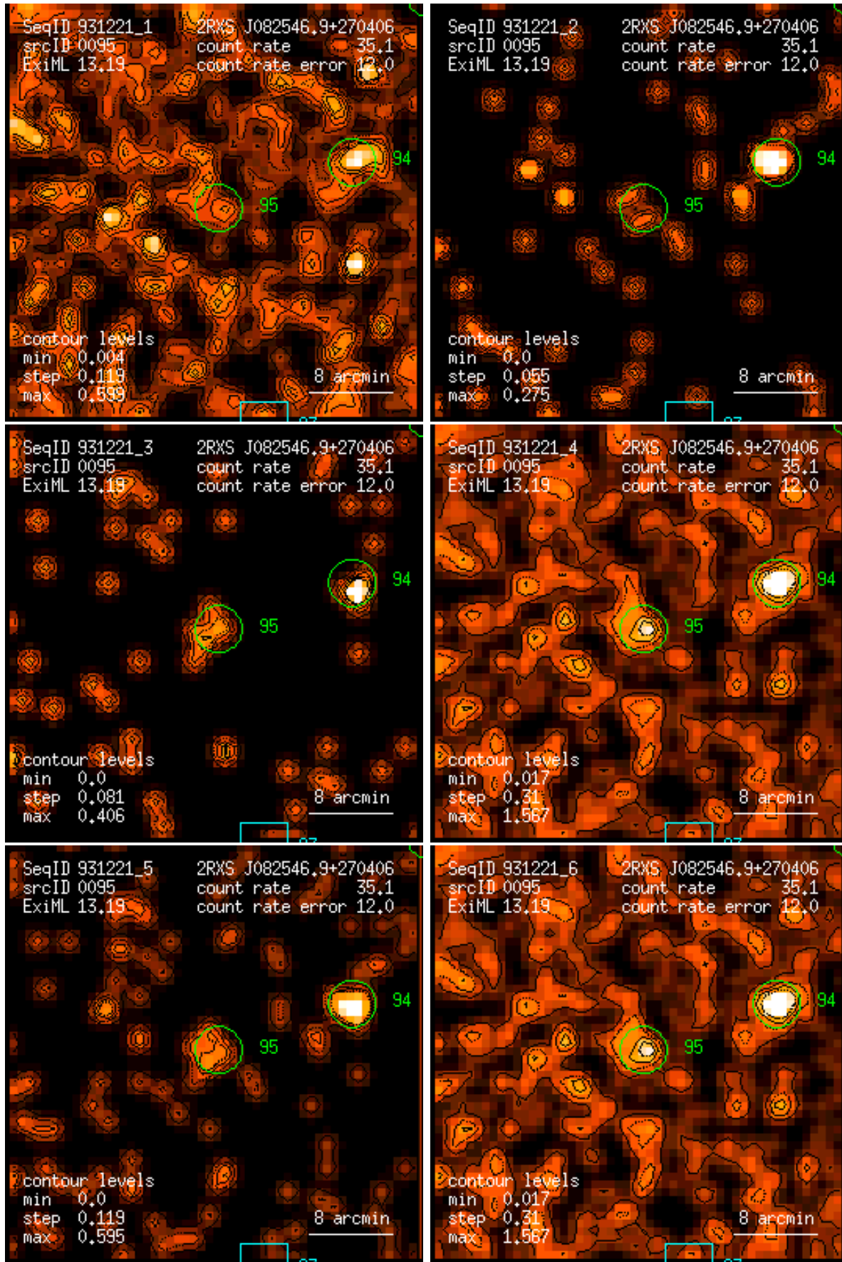
Figure 95: RASS 931221: detection 0095: band rate images, Gaussian filter: (1) PSPC channels 11 – 41, (2) 52 – 90, (3) 91 – 201, (4) 11 – 235, (5) 52 – 201, (6) 11 – 201. Broad band rates in counts/ks. Band rate contour levels in counts/ks/arcmin 2 .
