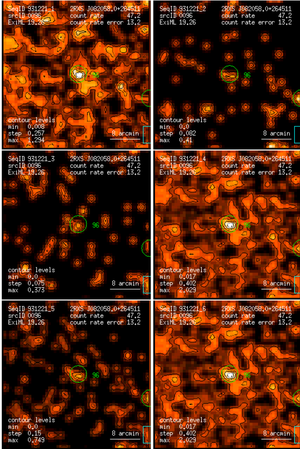
Figure 96: RASS 931221: detection 0096: band rate images, Gaussian filter: (1) PSPC channels 11 – 41, (2) 52 – 90, (3) 91 – 201, (4) 11 – 235, (5) 52 – 201, (6) 11 – 201. Broad band rates in counts/ks. Band rate contour levels in counts/ks/arcmin 2 .
