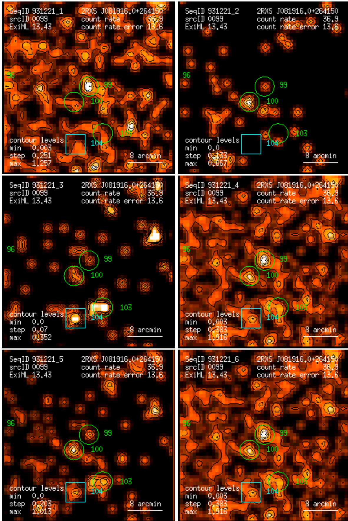
Figure 99: RASS 931221: detection 0099: band rate images, Gaussian filter: (1) PSPC channels 11 – 41, (2) 52 – 90, (3) 91 – 201, (4) 11 – 235, (5) 52 – 201, (6) 11 – 201. Broad band rates in counts/ks. Band rate contour levels in counts/ks/arcmin 2 .
